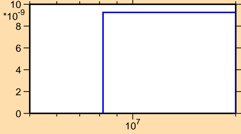
\sigma vs. E for ^{235}\text{Ra}(n,n\alpha)
