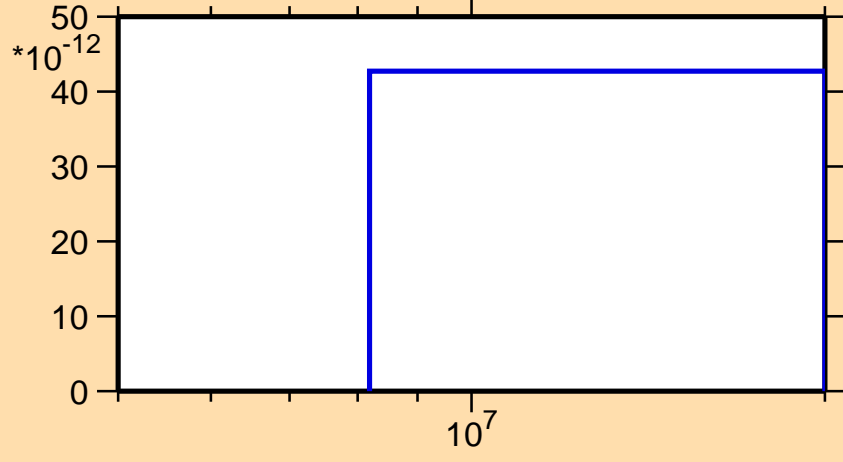
\sigma vs. E for ^{235}\text{Ra}(n,nt)
