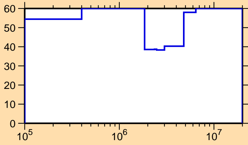
\Delta\sigma/\sigma vs. E for ^{235}\text{Ra}(n,\text{tot.})
