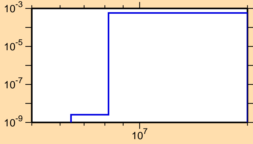
\sigma vs. E for ^{235}\text{Ra}(n,p)
