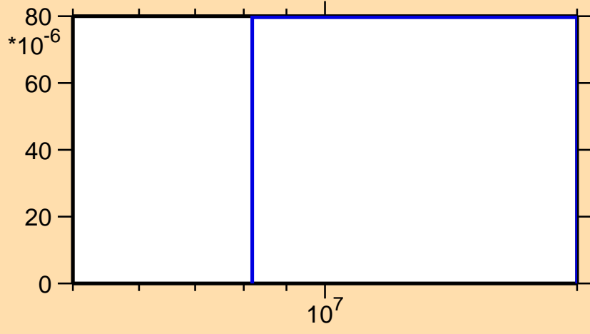
\sigma vs. E for ^{235}\text{Ra}(n,np)
