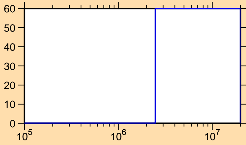
\Delta\sigma/\sigma vs. E for ^{235}\text{Ra}(n,f)
