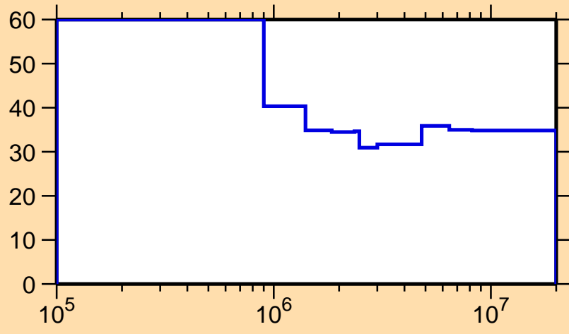
\Delta\sigma/\sigma vs. E for ^{235}\text{Ra}(n,\text{nonel.})
