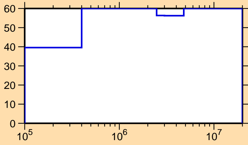
\Delta\sigma/\sigma vs. E for ^{235}\text{Ra}(n,\text{el.})
