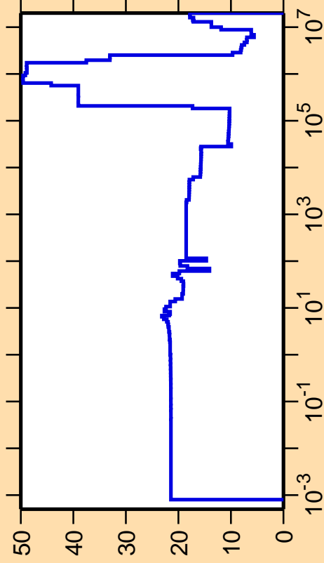
\Delta\sigma/\sigma vs. E for ^{75}\text{Rb}(n,\text{el.})
