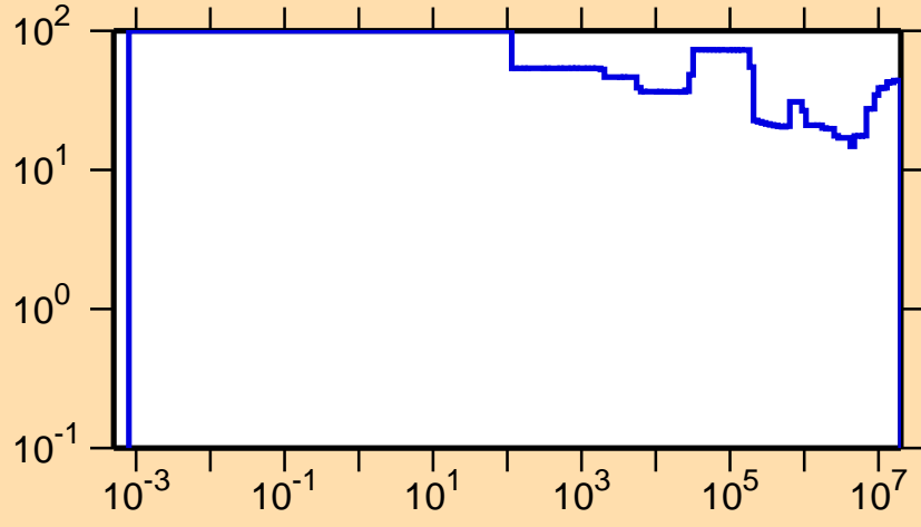
\Delta\sigma/\sigma vs. E for ^{75}\text{Rb}(n,p)
