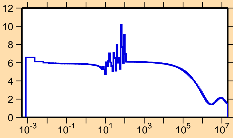
\sigma vs. E for ^{75}\text{Rb}(n,\text{el.})
