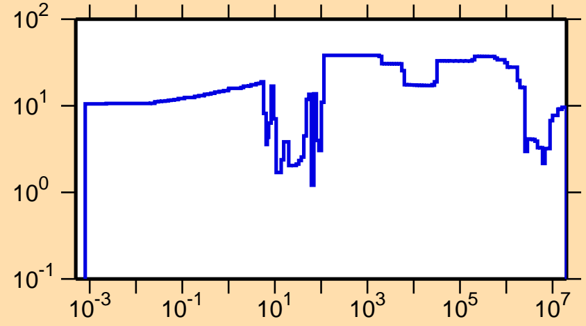
\Delta\sigma/\sigma vs. E for ^{75}\text{Rb}(n,\text{tot.})
