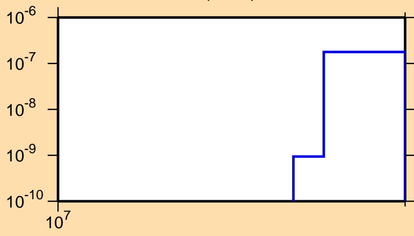
\sigma vs. E for ^{75}\text{Rb}(n,\text{nd})
