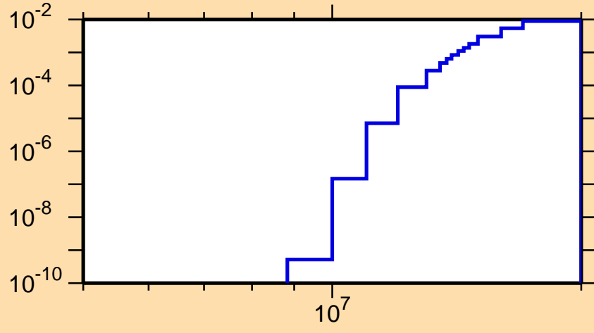
\sigma vs. E for ^{75}\text{Rb}(n,\text{pd})
