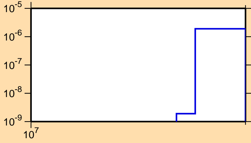
\sigma vs. E for ^{75}\text{Rb}(n,\text{pt})
