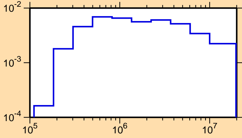
\sigma vs. E for ^{75}\text{Rb}(n,n_2)
