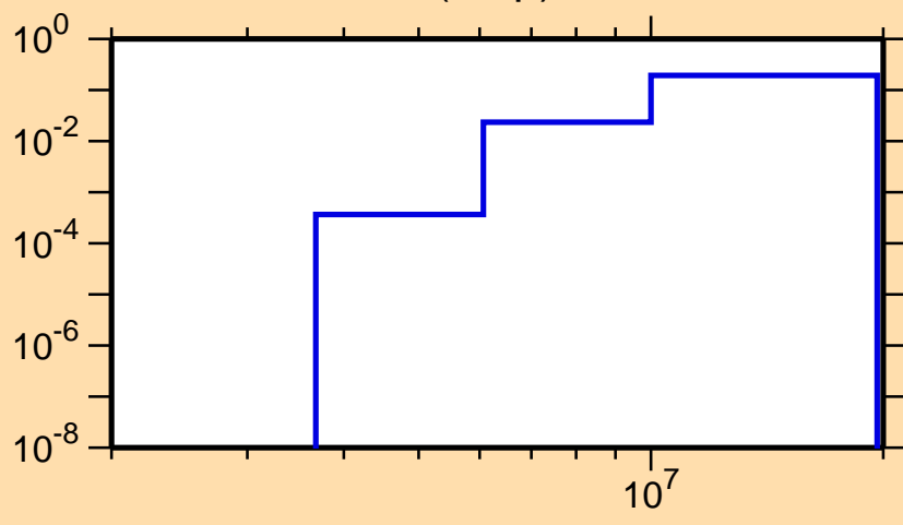
\sigma vs. E for ^{75}\text{Rb}(n,np)
