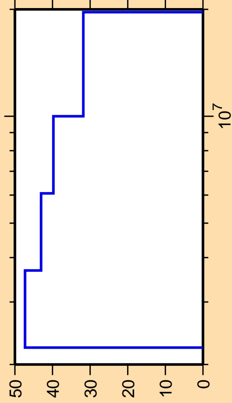
\Delta\sigma/\sigma vs. E for ^{75}\text{Rb}(n,np)
