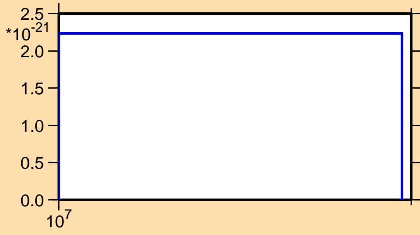
\sigma vs. E for ^{75}\text{Rb}(n,nt)
