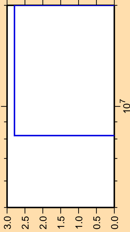
\Delta\sigma/\sigma vs. E for ^{75}\text{Rb} (mt 34)
