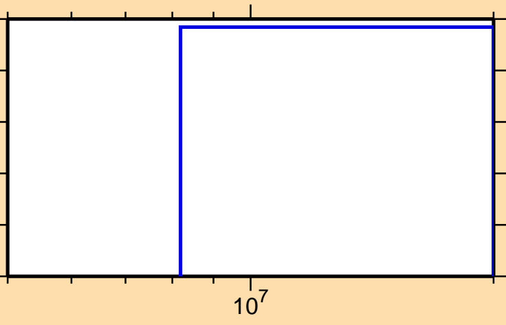
\sigma vs. E for ^{75}\text{Rb}(\text{mt117})
