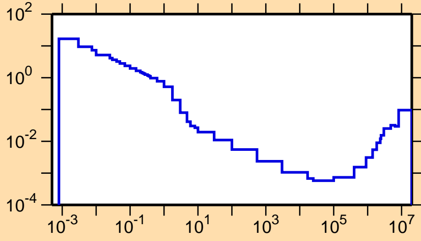
\sigma vs. E for ^{75}\text{Rb}(n,\alpha)
