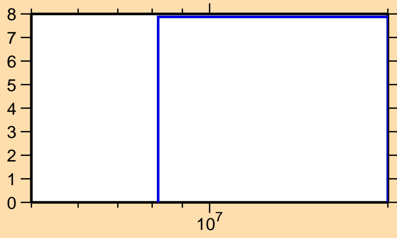
\Delta\sigma/\sigma vs. E for ^{75}\text{Rb}(n,\text{tot.})
