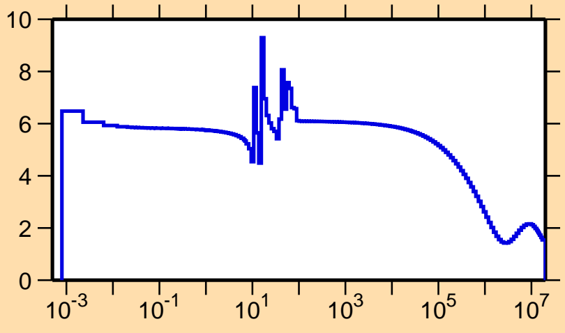
\sigma vs. E for ^{76}\text{Rb}(n,\text{el.})
