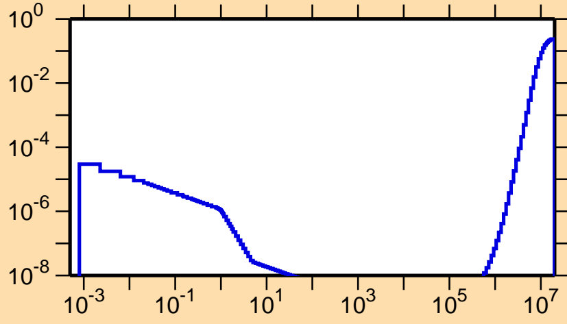
\sigma vs. E for ^{76}\text{Rb}(n,p\alpha)
