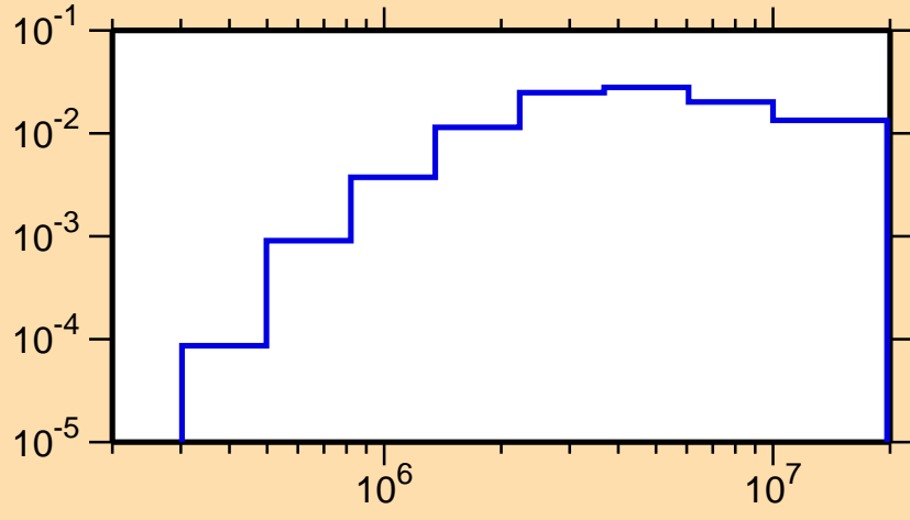
\sigma vs. E for ^{76}\text{Rb}(n,n_3)
