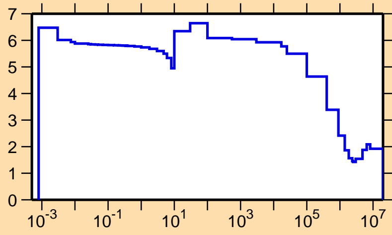
\sigma vs. E for ^{76}\text{Rb}(n,\text{el.})
