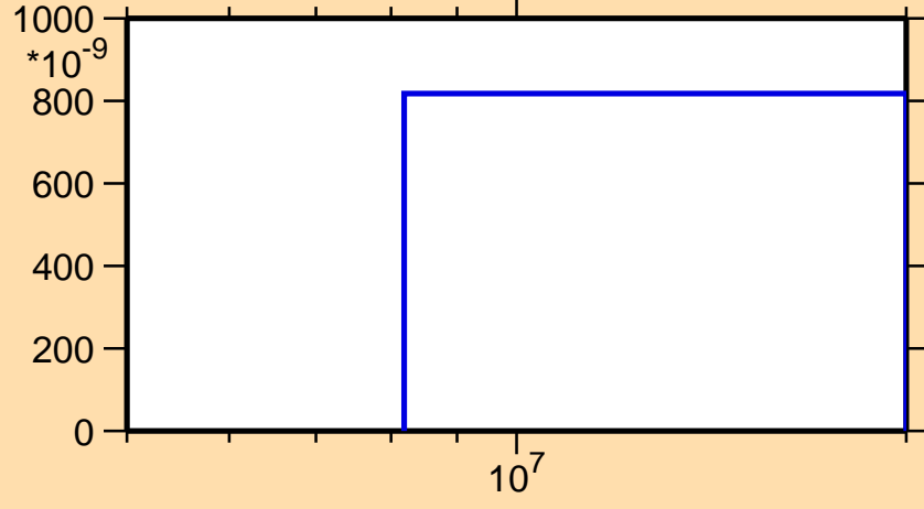
\sigma vs. E for ^{76}\text{Rb}(n,\text{nd})
