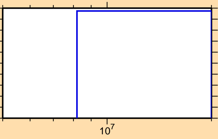
\sigma vs. E for ^{76}\text{Rb}(\text{mt117})
