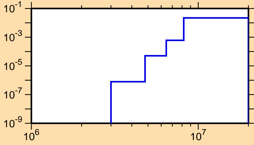
\sigma vs. E for ^{76}\text{Rb}(n,d)
