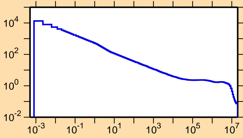
\sigma vs. E for ^{77}\text{Rb}(n,p)
