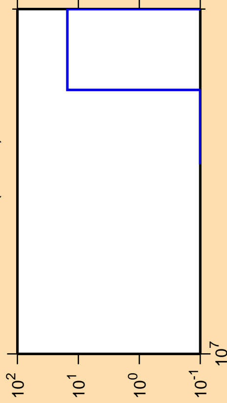
\Delta\sigma/\sigma vs. E for ^{77}\text{Rb} (mt 34)
