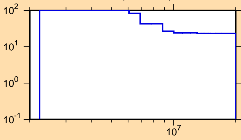
\Delta\sigma/\sigma vs. E for ^{77}\text{Rb}(n,ncont.)
