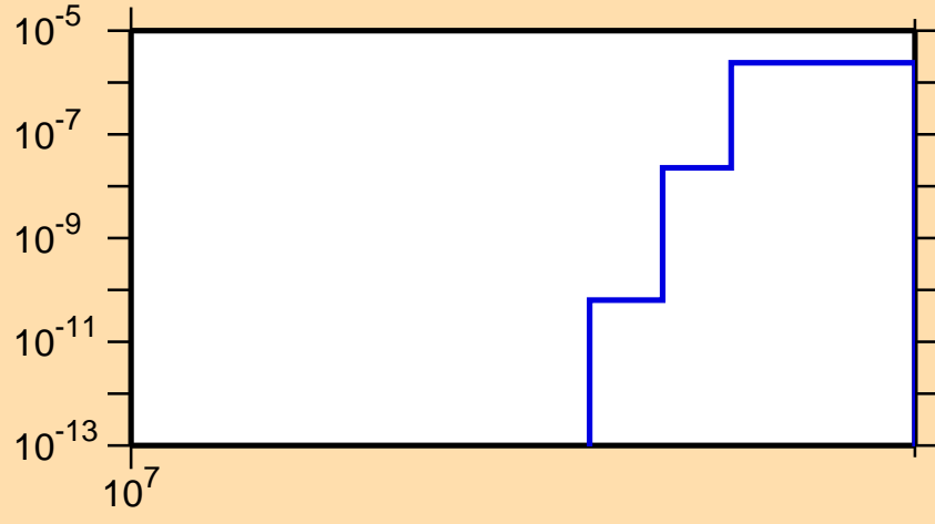
\sigma vs. E for ^{77}\text{Rb}(n,\text{nd})
