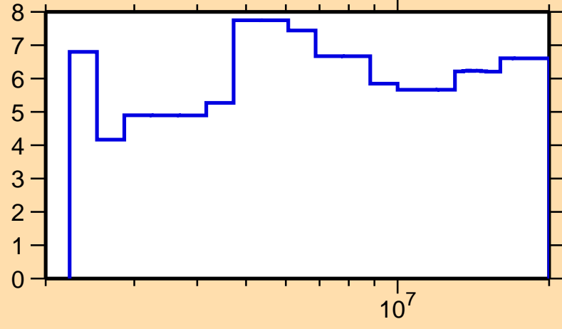
\Delta\sigma/\sigma vs. E for ^{77}\text{Rb}(n,n\text{onel.})
