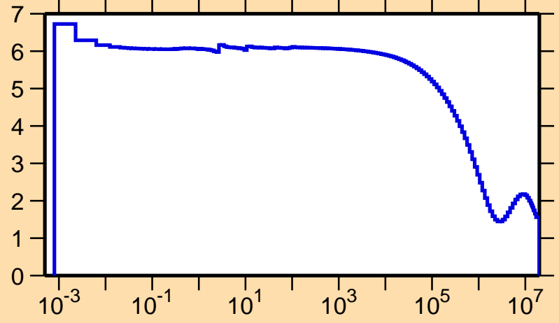
\sigma vs. E for ^{77}\text{Rb}(n,\text{el.})
