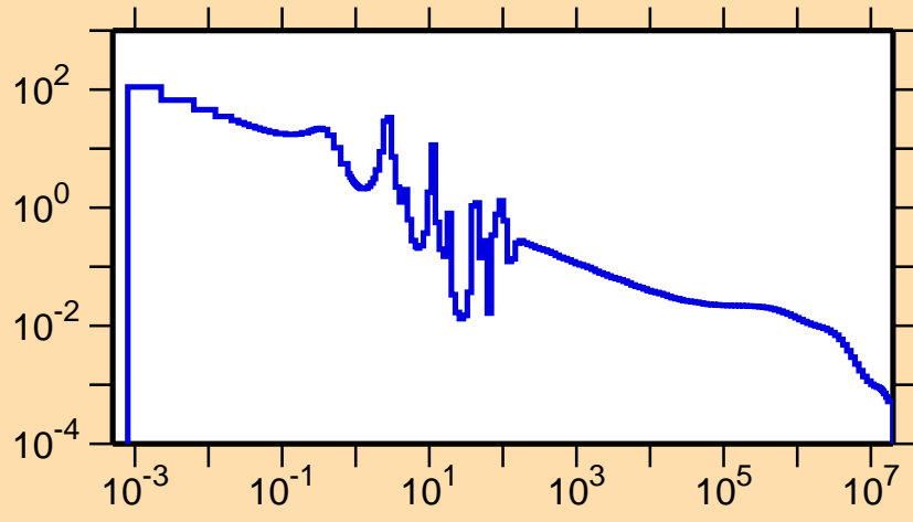
\sigma vs. E for ^{77}\text{Rb}(n,\gamma)
