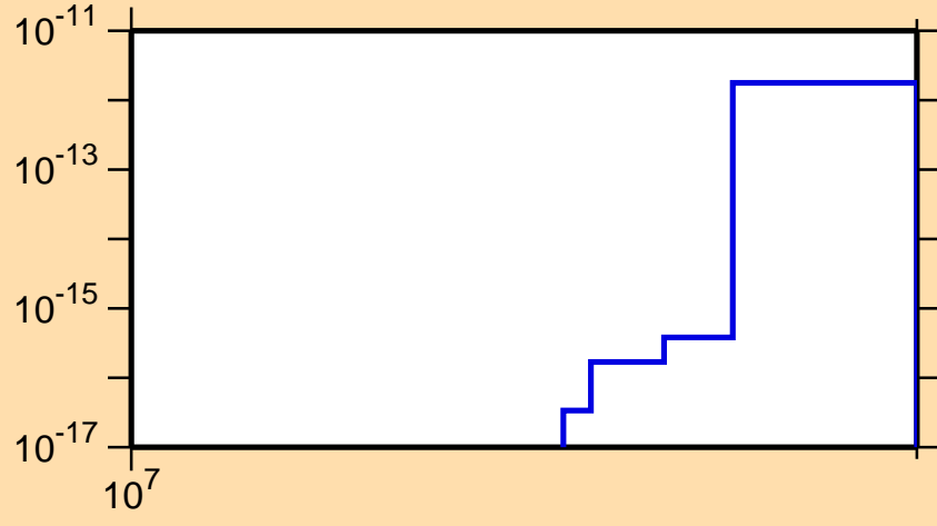
\sigma vs. E for ^{77}\text{Rb} (mt 34)
