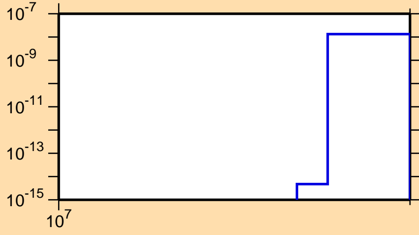
\sigma vs. E for ^{77}\text{Rb}(n,pt)
