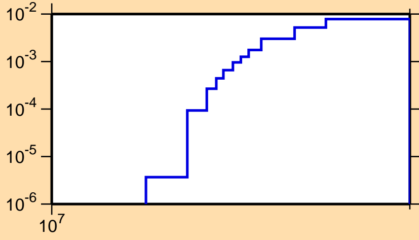
\sigma vs. E for ^{77}\text{Rb}(n,2n)
