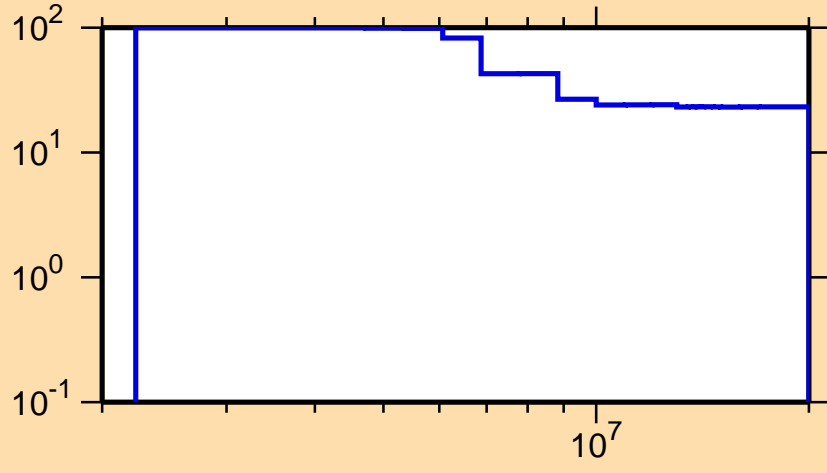
\Delta\sigma/\sigma vs. E for ^{77}\text{Rb}(n,n\text{cont.})
