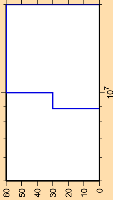
\Delta\sigma/\sigma vs. E for ^{77}\text{Rb}(n,t)
