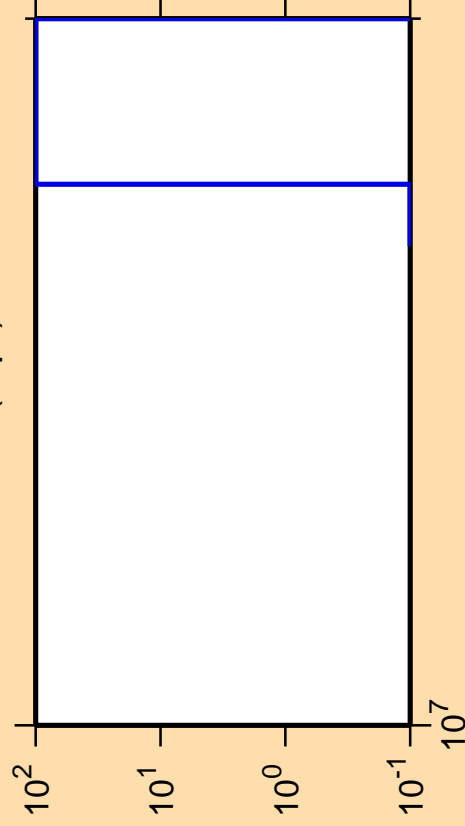
\Delta\sigma/\sigma vs. E for ^{77}\text{Rb}(n,pt)
