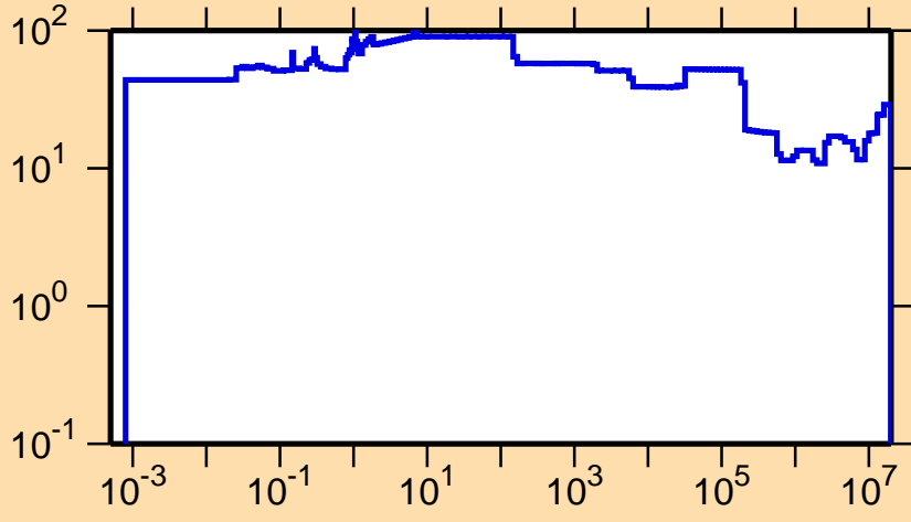
\Delta\sigma/\sigma vs. E for ^{77}\text{Rb}(n,p)
