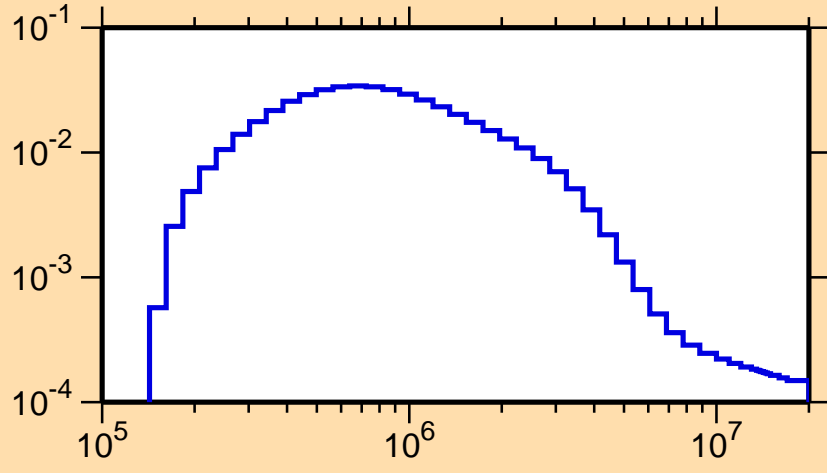
\sigma vs. E for ^{77}\text{Rb}(n,n_1)
