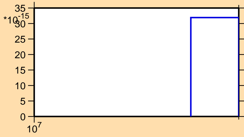
\sigma vs. E for ^{77}\text{Rb}(n,nt)
