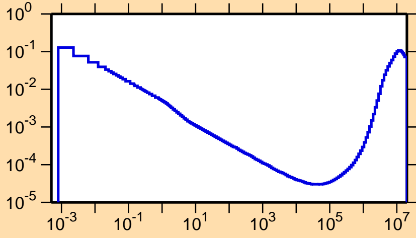
\sigma vs. E for ^{77}\text{Rb}(n,\alpha)
