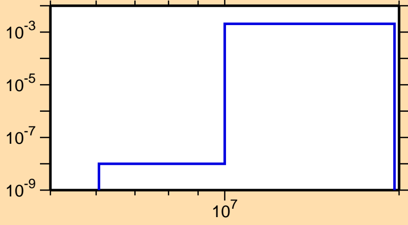
\sigma vs. E for ^{77}\text{Rb}(n,n\alpha)
