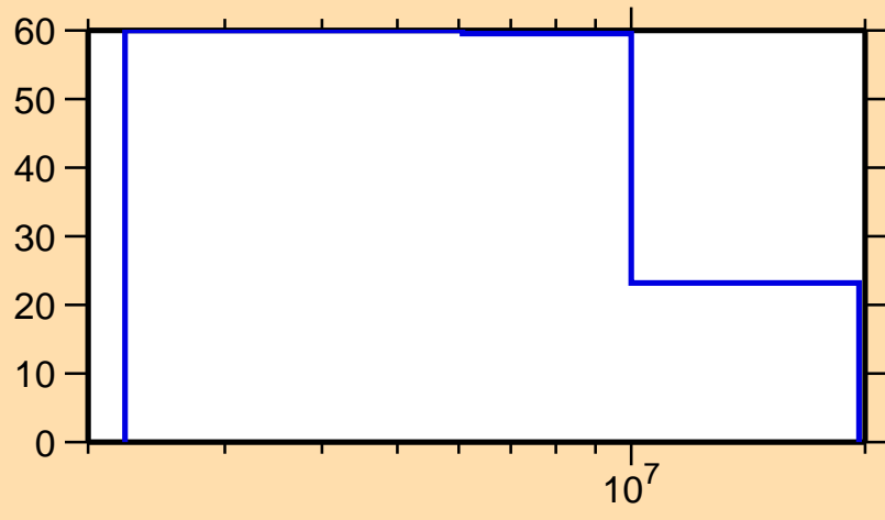
\Delta\sigma/\sigma vs. E for ^{77}\text{Rb}(n,ncont.)
