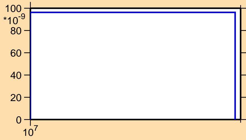
\sigma vs. E for ^{77}\text{Rb}(n,2np)
