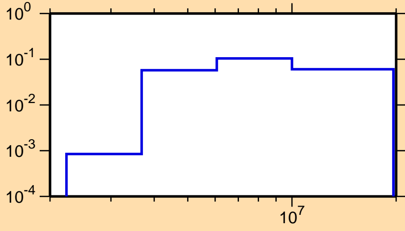
\sigma vs. E for ^{77}\text{Rb}(n,n\text{cont.})
