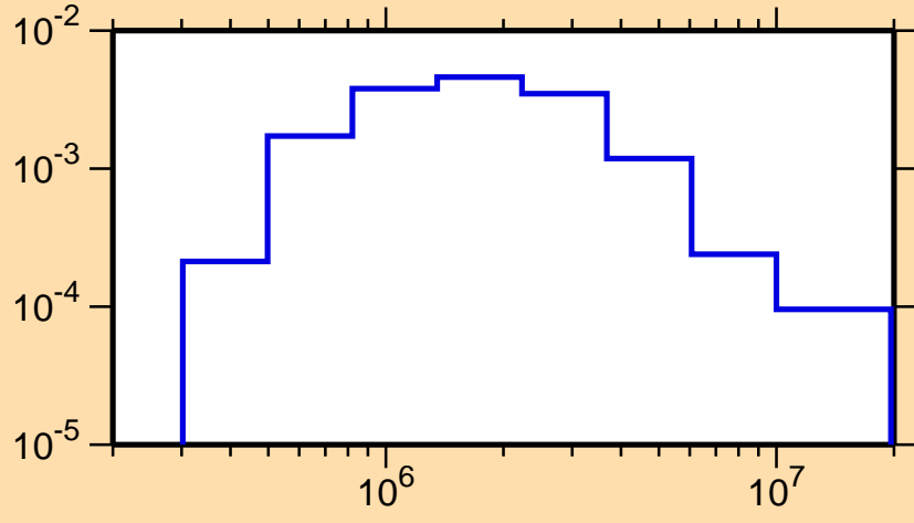
\sigma vs. E for ^{77}\text{Rb}(n,n_4)
