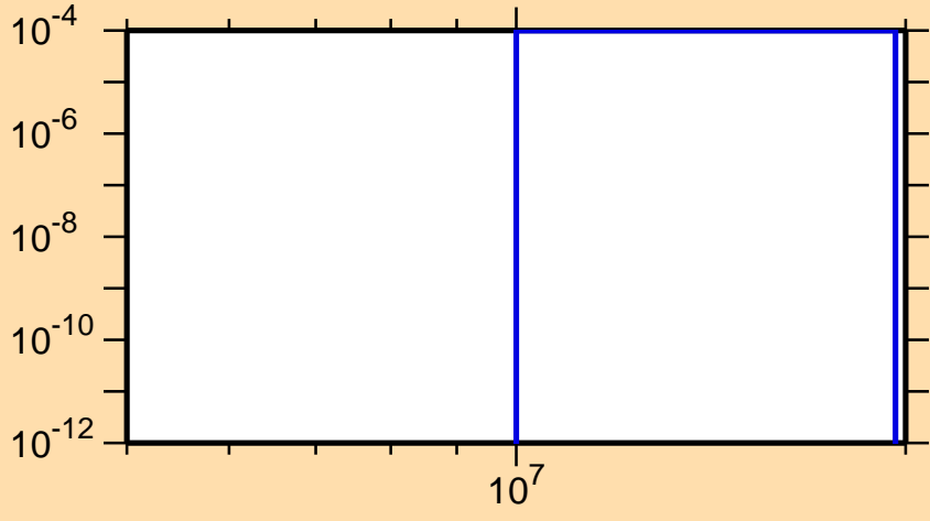
\sigma vs. E for ^{77}\text{Rb}(n,\text{pd})
