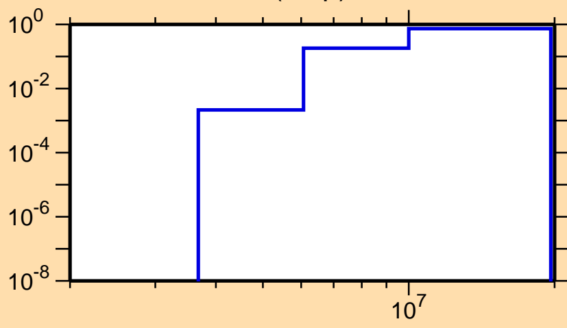
\sigma vs. E for ^{77}\text{Rb}(n,np)
