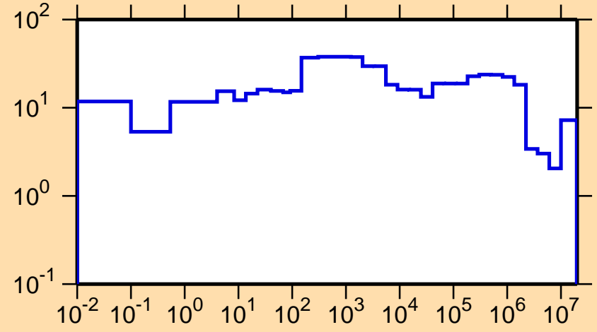
\Delta\sigma/\sigma vs. E for ^{77}\text{Rb}(n,\text{tot.})
