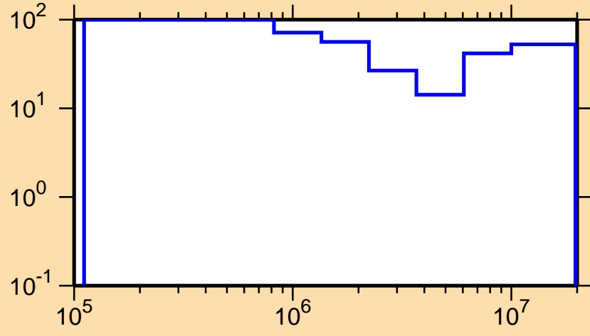
\Delta\sigma/\sigma vs. E for ^{77}\text{Rb}(n,n_1)
