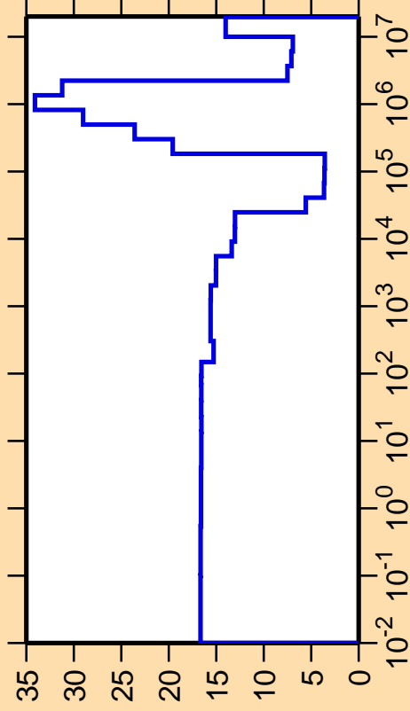
\Delta\sigma/\sigma vs. E for ^{77}\text{Rb}(n,\text{el.})
