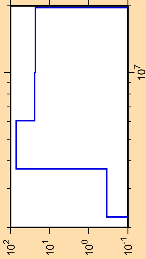
\Delta\sigma/\sigma vs. E for ^{77}\text{Rb}(n,np)
