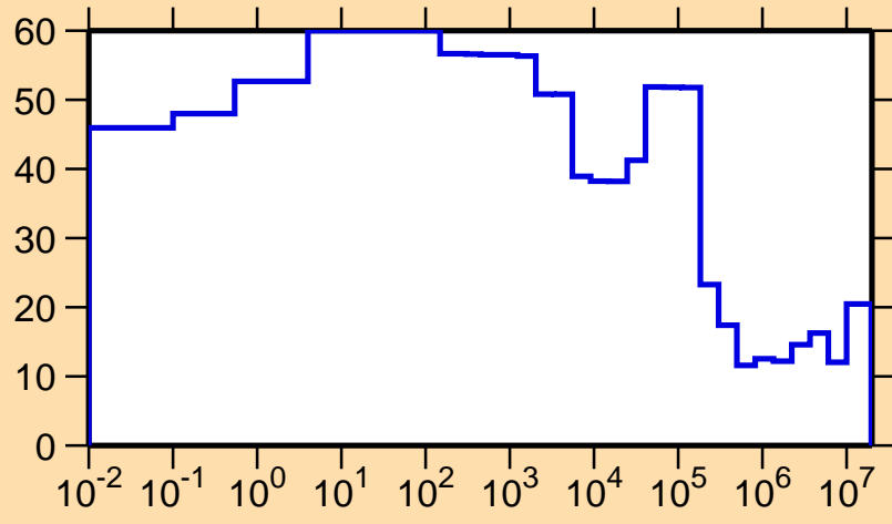
\Delta\sigma/\sigma vs. E for ^{77}\text{Rb}(n,p)
