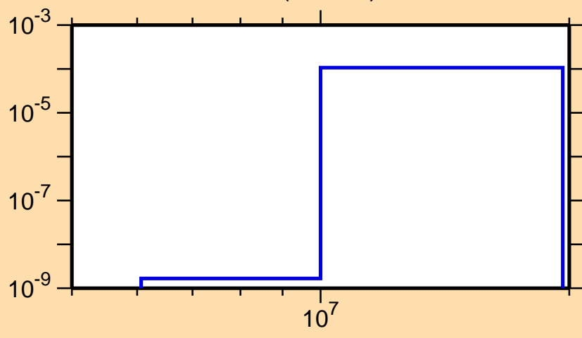
\sigma vs. E for ^{77}\text{Rb}(n,\text{He}3)
