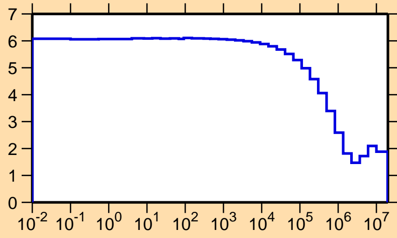
\sigma vs. E for ^{77}\text{Rb}(n,\text{el.})
