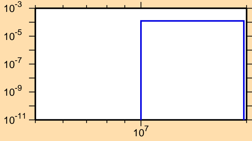
\sigma vs. E for ^{77}\text{Rb}(n,t)
