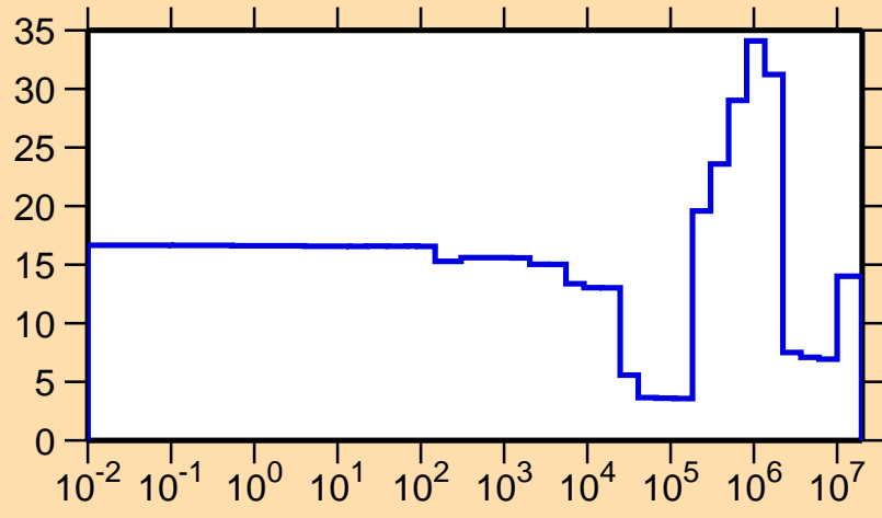
\Delta\sigma/\sigma vs. E for ^{77}\text{Rb}(n,\text{el.})
