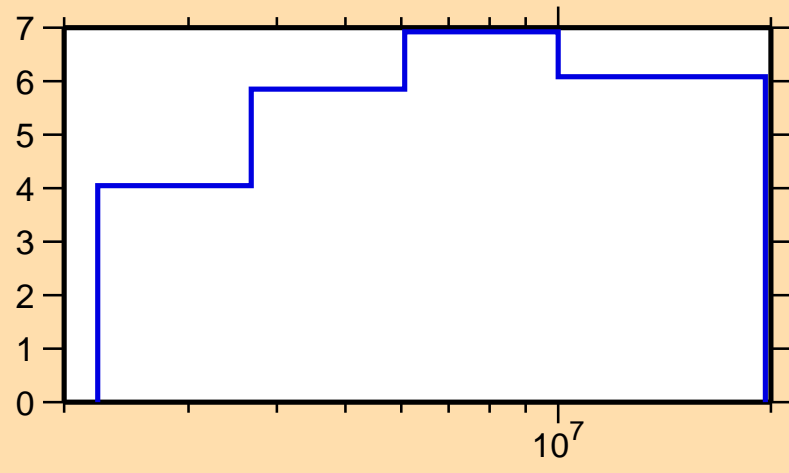
\Delta\sigma/\sigma vs. E for ^{77}\text{Rb}(n,n\text{nonel.})
