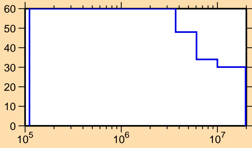
\Delta\sigma/\sigma vs. E for ^{77}\text{Rb}(n,\text{inel.})
