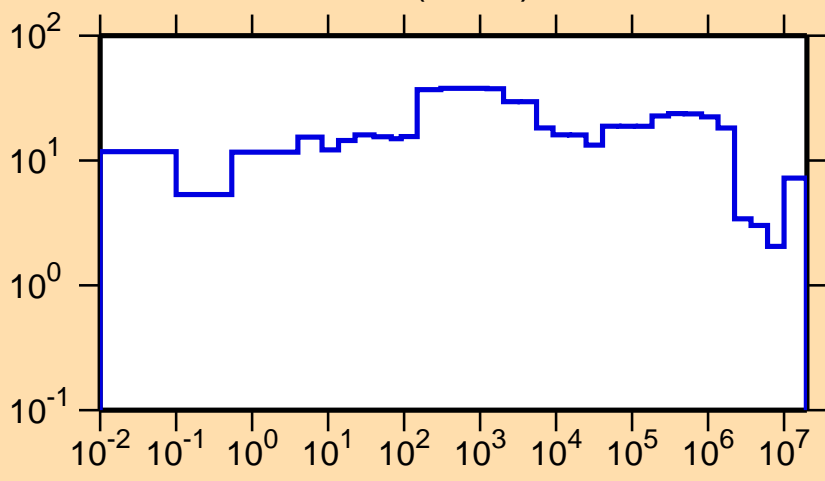
\Delta\sigma/\sigma vs. E for ^{77}\text{Rb}(n,\text{tot.})
