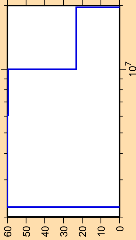
\Delta\sigma/\sigma vs. E for ^{77}\text{Rb}(n,n\text{cont.})
