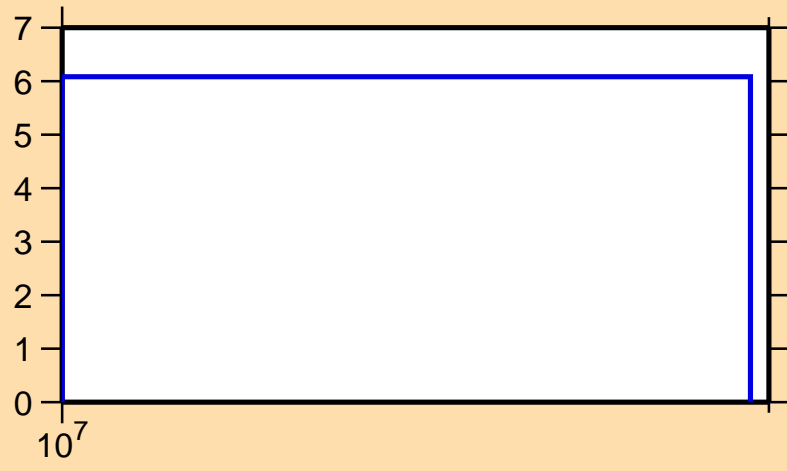
\Delta\sigma/\sigma vs. E for ^{77}\text{Rb}(n,\text{nonel.})
