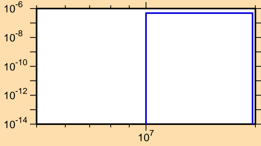
\sigma vs. E for ^{77}\text{Rb} (mt 45)
