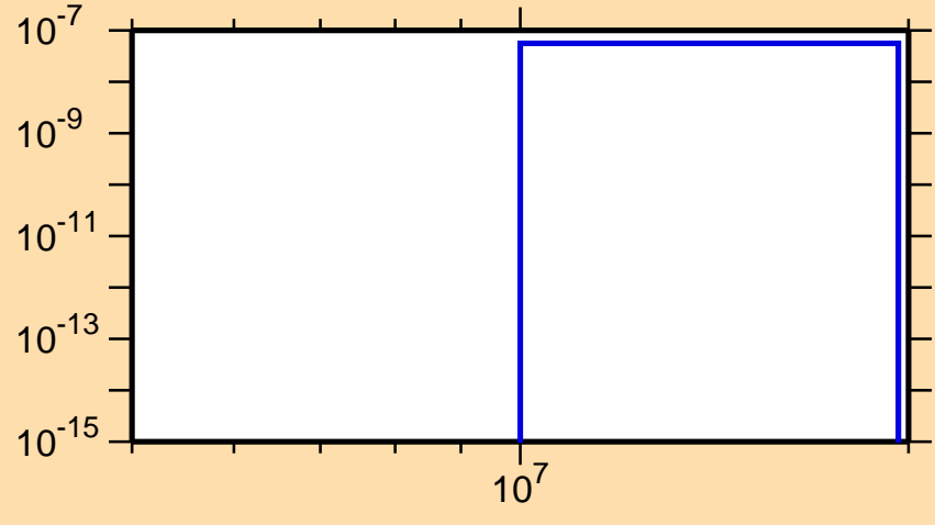
\sigma vs. E for ^{77}\text{Rb}(\text{mt117})
