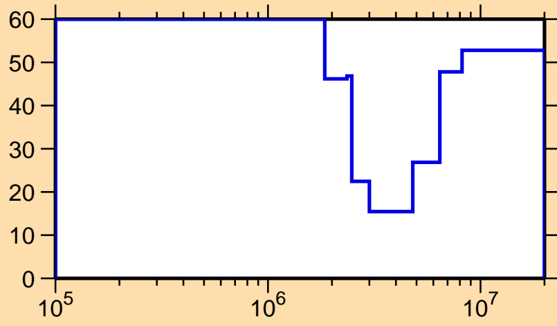
\Delta\sigma/\sigma vs. E for ^{77}\text{Rb}(n,n_1)
