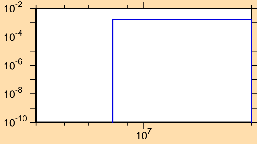
\sigma vs. E for ^{77}\text{Rb}(n,n\alpha)
