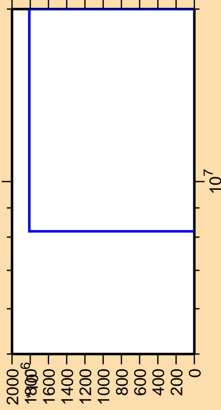
\Delta\sigma/\sigma vs. E for ^{77}\text{Rb}(n,nt)
