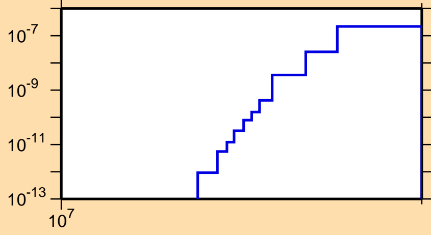
\sigma vs. E for ^{78}\text{Rb} (mt117)
