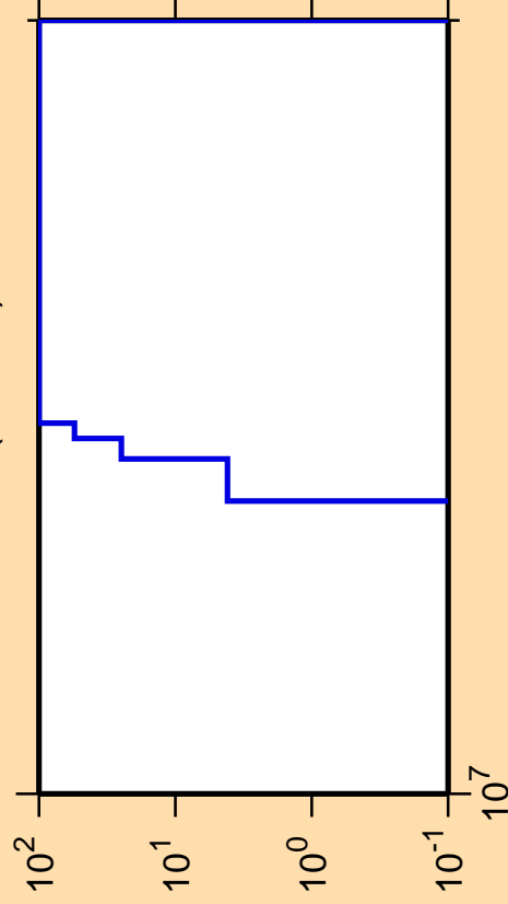
\Delta\sigma/\sigma vs. E for ^{78}\text{Rb} (mt117)
