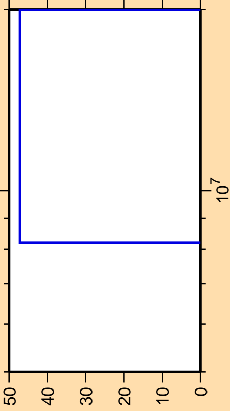
\Delta\sigma/\sigma vs. E for ^{78}\text{Rb}(n,n\text{cont.})
