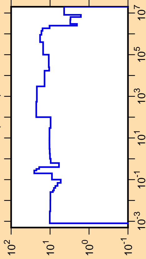
\Delta\sigma/\sigma vs. E for ^{78}\text{Rb}(n,\text{tot.})
