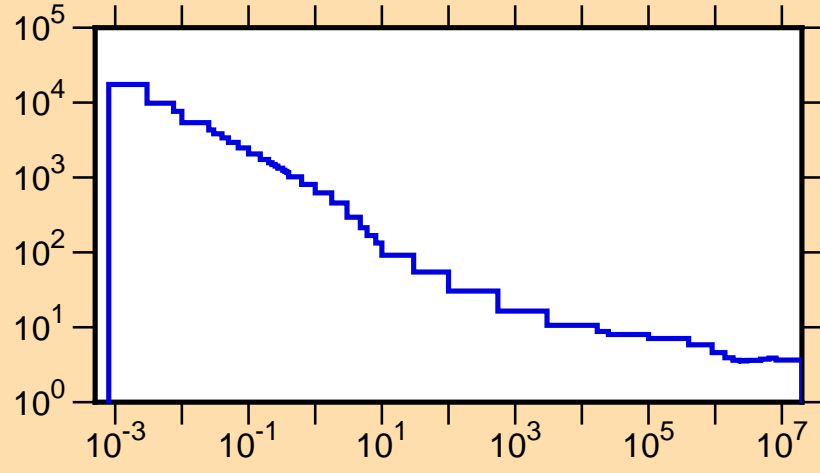
\sigma vs. E for ^{78}\text{Rb}(n,\text{tot.})
