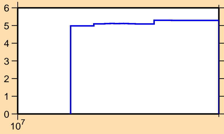
\Delta\sigma/\sigma vs. E for ^{79}\text{Rb}(n,\text{nonel.})
