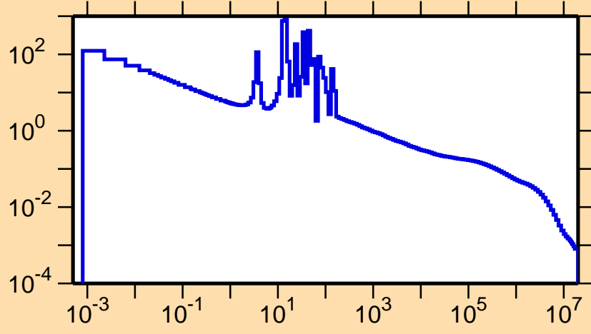
\sigma vs. E for ^{79}\text{Rb}(n,\gamma)
