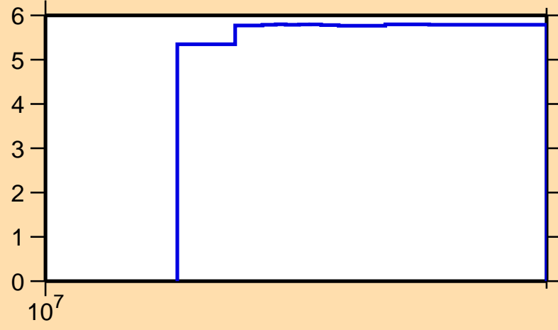
\Delta\sigma/\sigma vs. E for ^{79}\text{Rb}(n,\text{el.})
