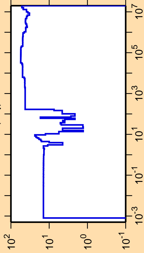
\Delta\sigma/\sigma vs. E for ^{79}\text{Rb}(n,\gamma)
