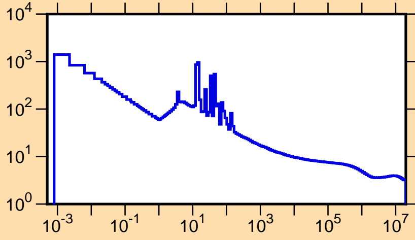
\sigma vs. E for ^{79}\text{Rb}(n,\text{tot.})
