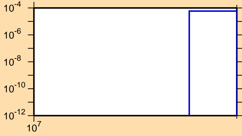
\sigma vs. E for ^{79}\text{Rb}(n,2np)
