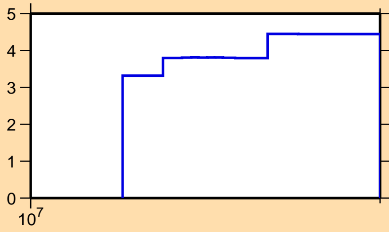
\Delta\sigma/\sigma vs. E for ^{79}\text{Rb}(n,\text{tot.})
