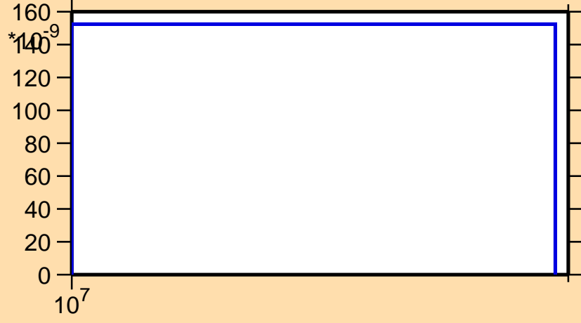
\sigma vs. E for ^{79}\text{Rb}(n,\text{nd})
