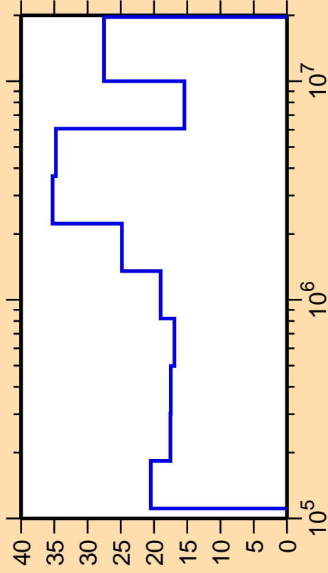
\Delta\sigma/\sigma vs. E for ^{79}\text{Rb}(n,n_4)
