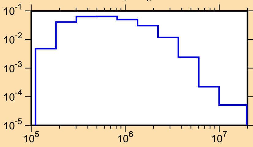
\sigma vs. E for ^{79}\text{Rb}(n,n_4)
