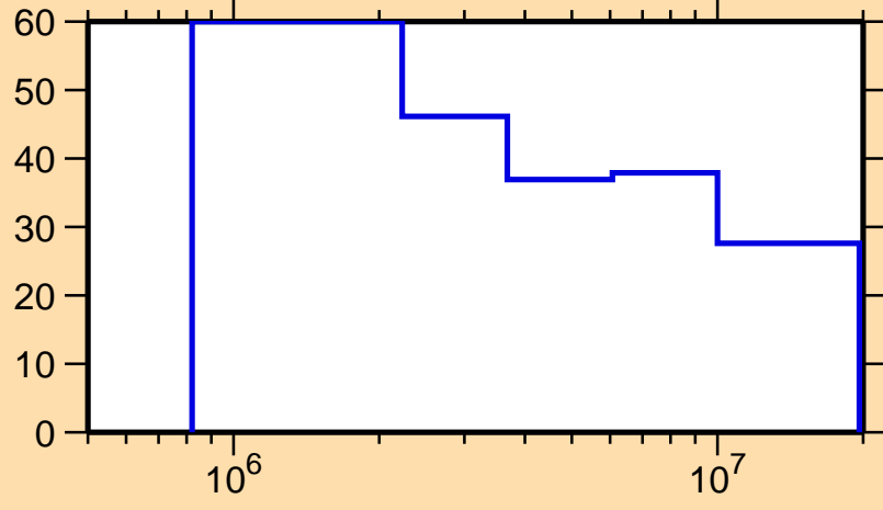
\Delta\sigma/\sigma vs. E for ^{79}\text{Rb}(n,n\text{cont.})
