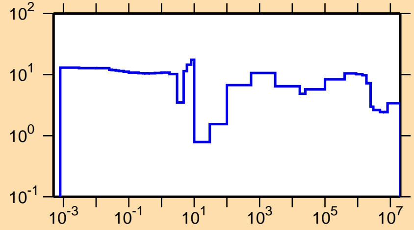
\Delta\sigma/\sigma vs. E for ^{79}\text{Rb}(n,\text{tot.})
