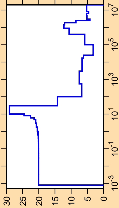
\Delta\sigma/\sigma vs. E for ^{79}\text{Rb}(n,\text{el.})
