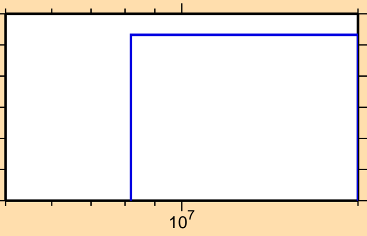
\sigma vs. E for ^{79}\text{Rb}(n,\text{pd})
