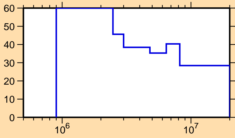
\Delta\sigma/\sigma vs. E for ^{79}\text{Rb}(n,ncont.)
