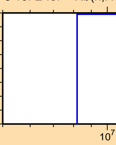
\sigma vs. E for ^{79}\text{Rb}(n,\text{He3})
