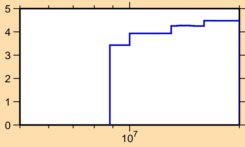
\Delta\sigma/\sigma vs. E for ^{80}\text{Rb}(n,\text{tot.})
