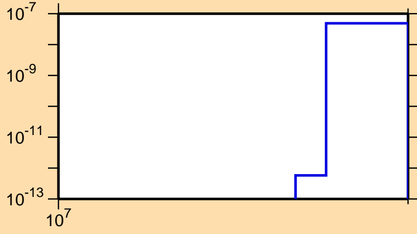
\sigma vs. E for ^{80}\text{Rb}(n,pt)
