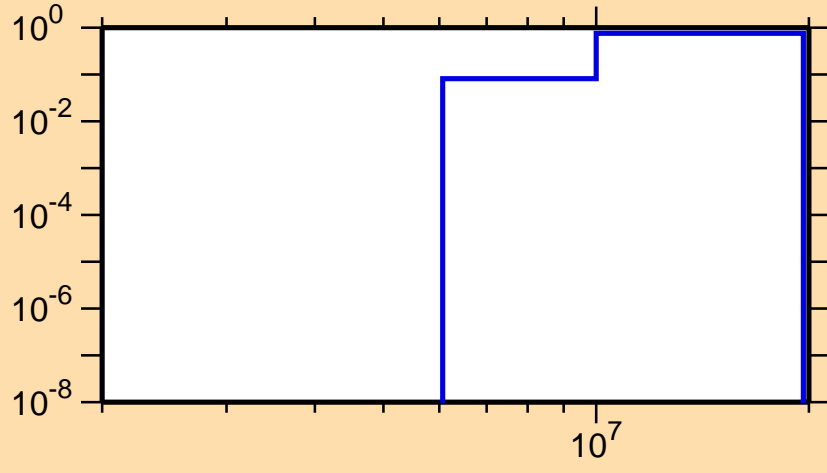
\sigma vs. E for ^{80}\text{Rb}(n,np)
