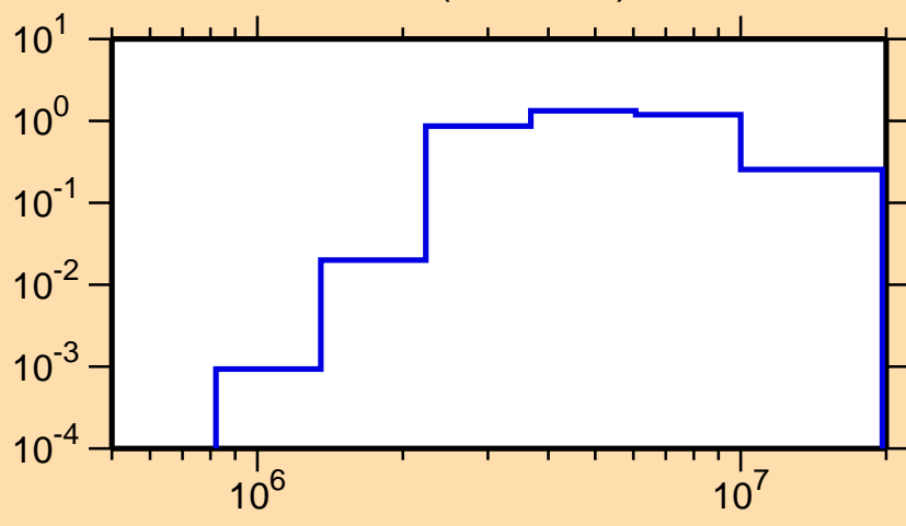
\sigma vs. E for ^{80}\text{Rb}(n,n\text{cont.})
