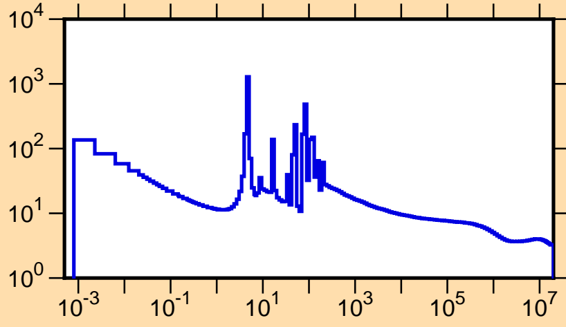
\sigma vs. E for ^{81}\text{Rb}(n,\text{tot.})
