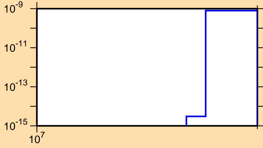
\sigma vs. E for ^{81}\text{Rb}(n,nt)
