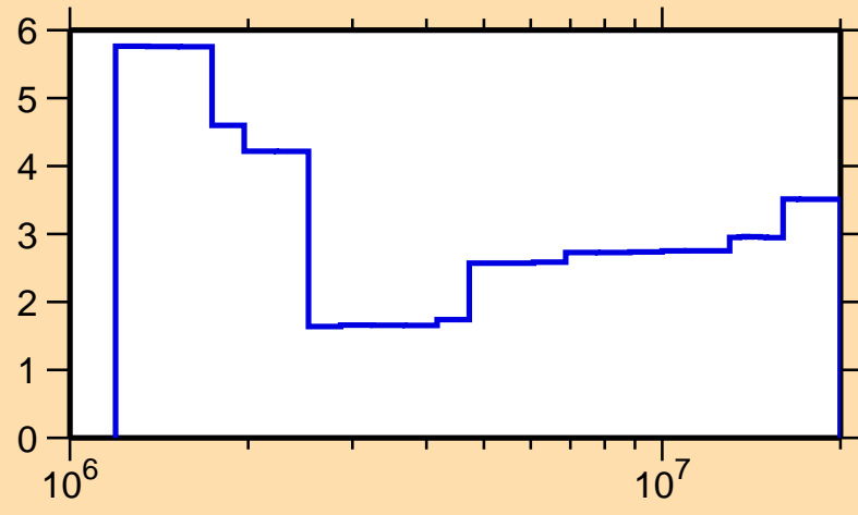
\Delta\sigma/\sigma vs. E for ^{81}\text{Rb}(n,n\text{onel.})
