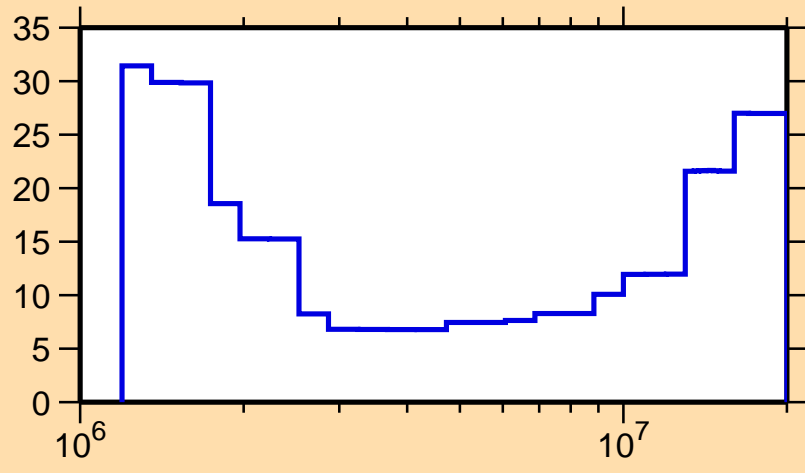
\Delta\sigma/\sigma vs. E for ^{81}\text{Rb}(n,n\text{cont.})
