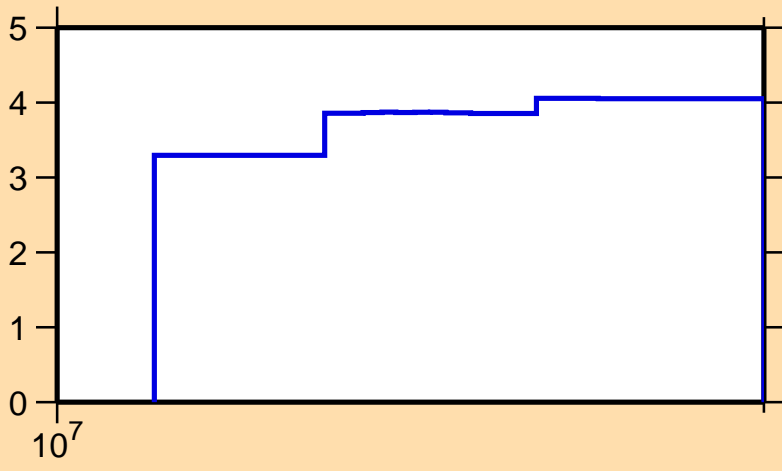
\Delta\sigma/\sigma vs. E for ^{81}\text{Rb}(n,\text{el.})
