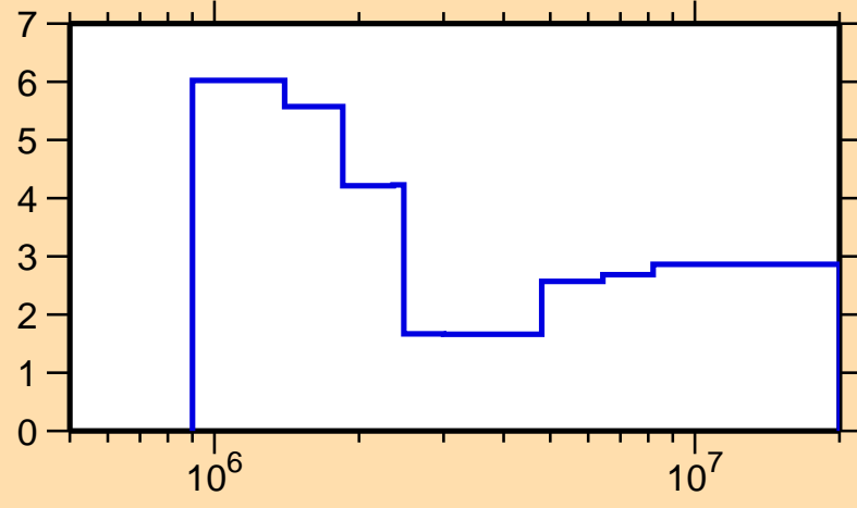
\Delta\sigma/\sigma vs. E for ^{81}\text{Rb}(n,n\text{nonel.})
