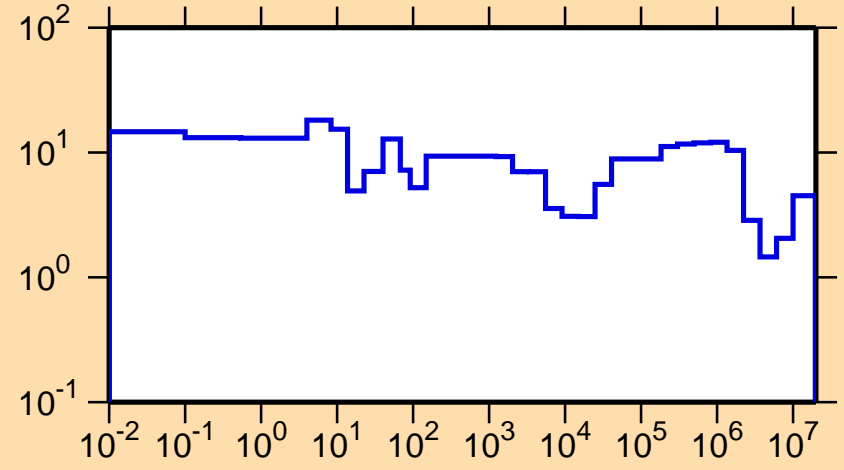
\Delta\sigma/\sigma vs. E for ^{82}\text{Rb}(n,\text{tot.})
