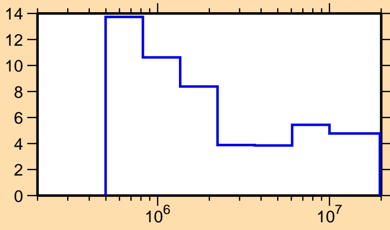
\Delta\sigma/\sigma vs. E for ^{82}\text{Rb}(n,n\text{nonel.})
