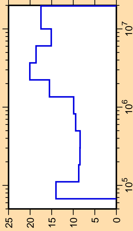
\Delta\sigma/\sigma vs. E for ^{82}\text{Rb}(n,n_2)
