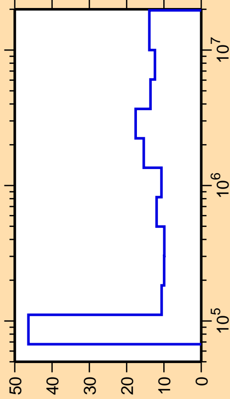
\Delta\sigma/\sigma vs. E for ^{82}\text{Rb}(n,n_1)
