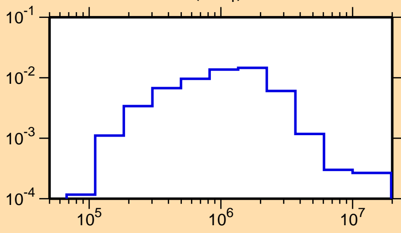
\sigma vs. E for ^{82}\text{Rb}(n,n_1)
