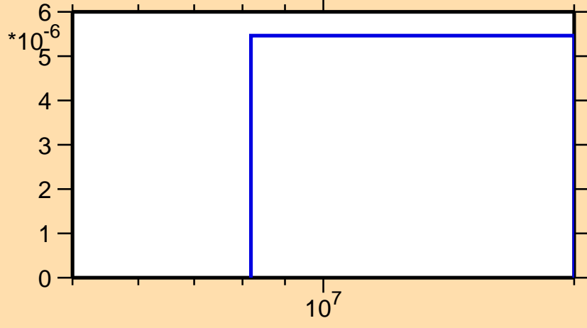
\sigma vs. E for ^{82}\text{Rb}(n,\text{nd})
