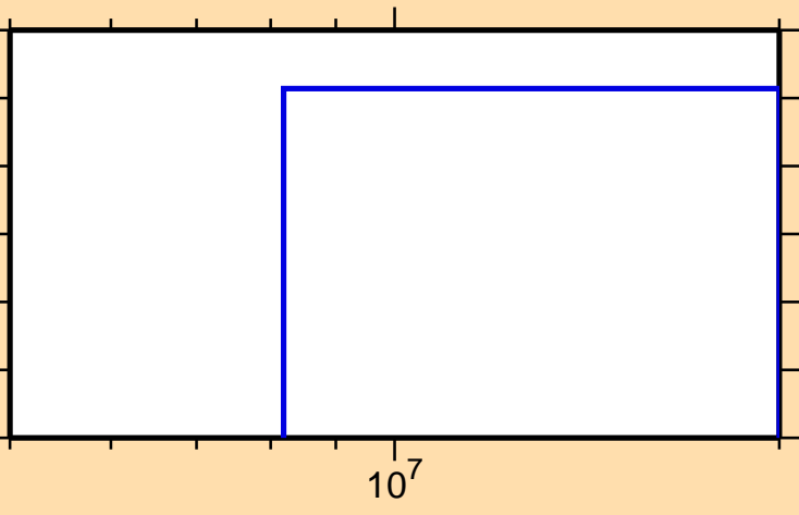
\sigma vs. E for ^{82}\text{Rb}(n,2np)
