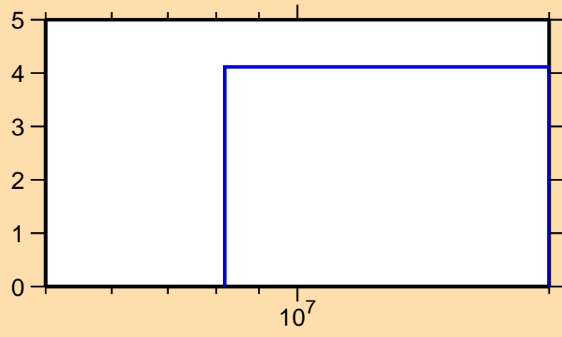
\Delta\sigma/\sigma vs. E for ^{82}\text{Rb}(n,\text{tot.})
