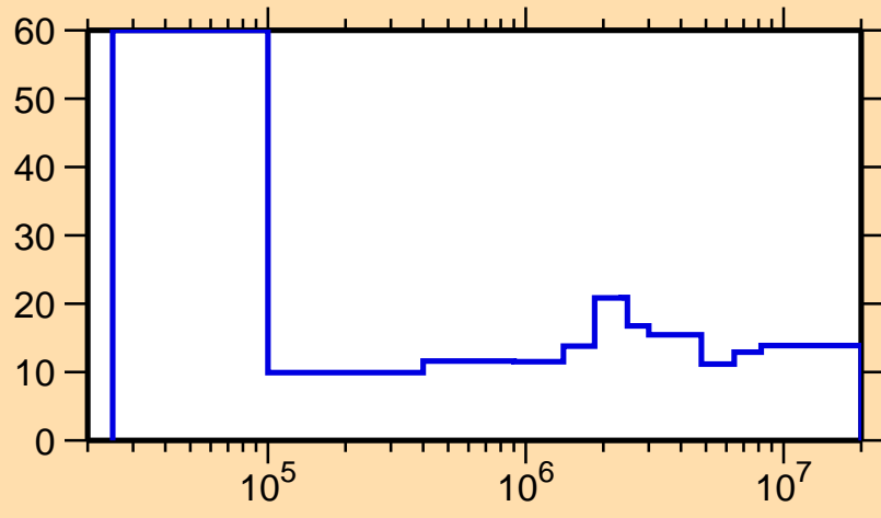
\Delta\sigma/\sigma vs. E for ^{82}\text{Rb}(n,n_1)
