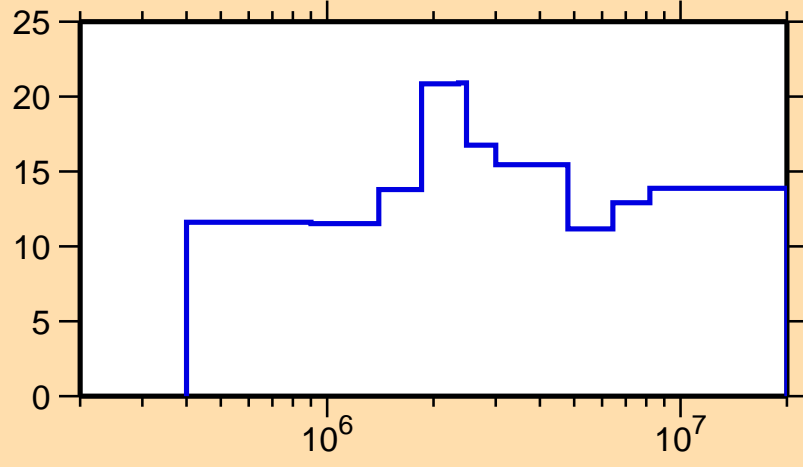
\Delta\sigma/\sigma vs. E for ^{82}\text{Rb}(n,n_1)
