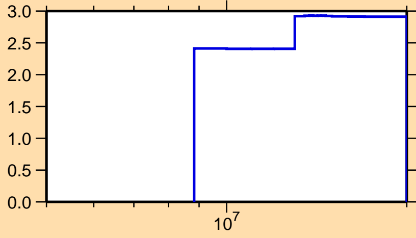
\Delta\sigma/\sigma vs. E for ^{84}\text{Rb}(n,\text{nonel.})
