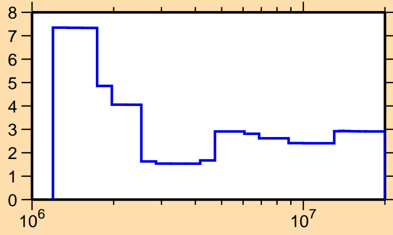
\Delta\sigma/\sigma vs. E for ^{84}\text{Rb}(n,\text{nonel.})
