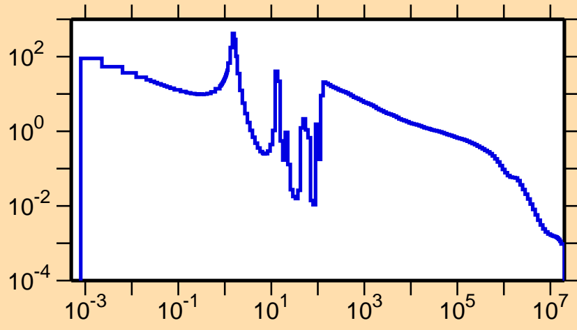
\sigma vs. E for ^{84}\text{Rb}(n,\gamma)
