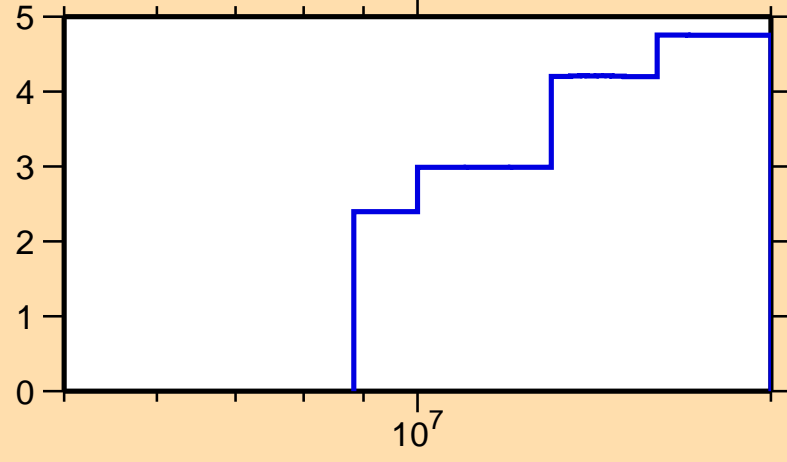
\Delta\sigma/\sigma vs. E for ^{84}\text{Rb}(n,\text{el.})
