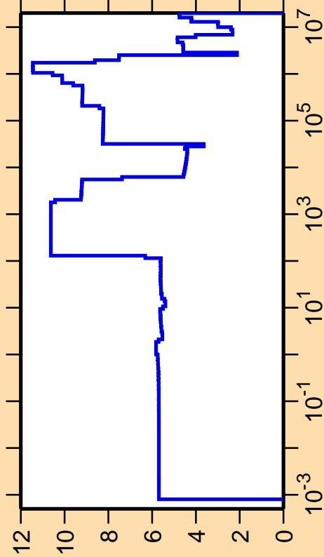
\Delta\sigma/\sigma vs. E for ^{84}\text{Rb}(n,\text{el.})
