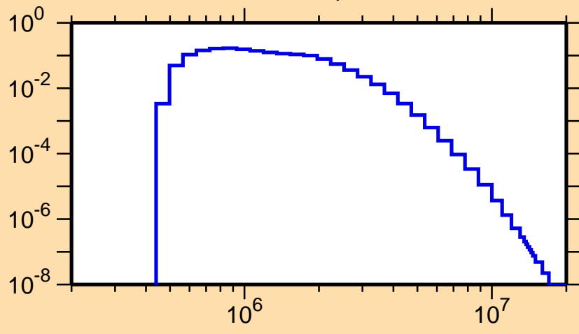
\sigma vs. E for ^{84}\text{Rb}(n,n_4)
