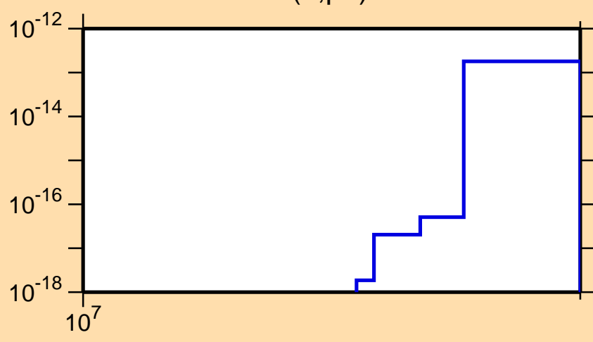
\sigma vs. E for ^{84}\text{Rb}(n,\text{pd})
