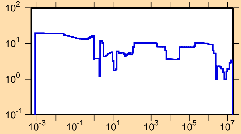
\Delta\sigma/\sigma vs. E for ^{84}\text{Rb}(n,\text{tot.})
