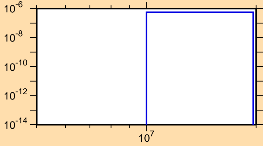
\sigma vs. E for ^{84}\text{Rb}(n,p\alpha)
