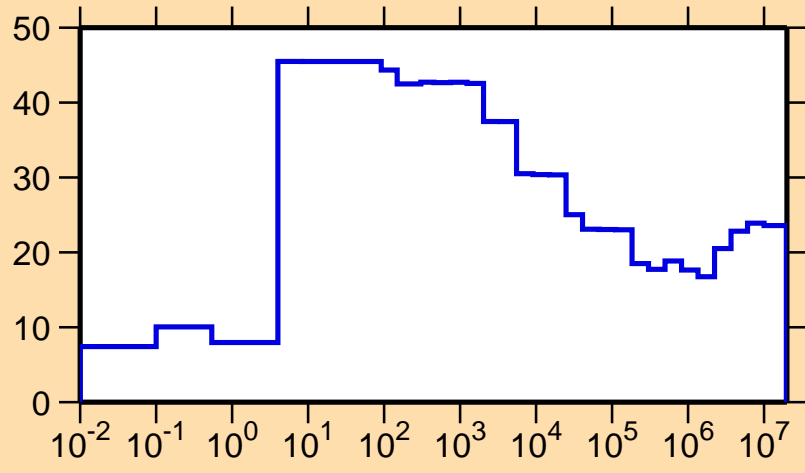
\Delta\sigma/\sigma vs. E for ^{84}\text{Rb}(n,p)
