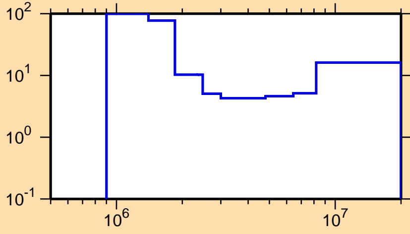
\Delta\sigma/\sigma vs. E for ^{84}\text{Rb}(n,n\text{cont.})
