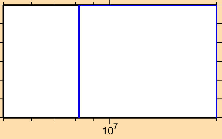
\sigma vs. E for ^{84}\text{Rb}(n,\text{He3})
