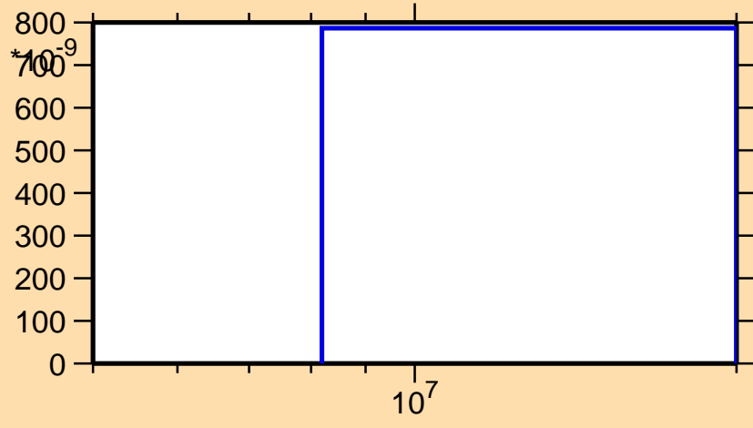
\sigma vs. E for ^{84}\text{Rb}(n,\text{nd})
