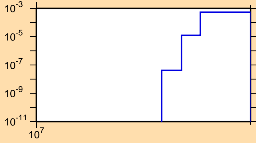
\sigma vs. E for ^{84}\text{Rb}(n,2np)
