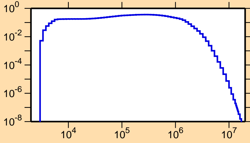
\sigma vs. E for ^{84}\text{Rb}(n,n_3)
