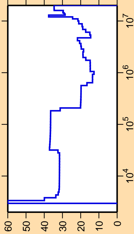
\Delta\sigma/\sigma vs. E for ^{84}\text{Rb}(n,n_3)
