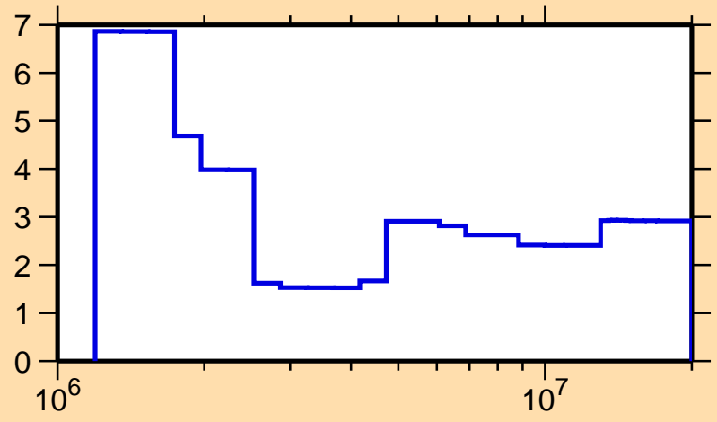
\Delta\sigma/\sigma vs. E for ^{84}\text{Rb}(n,n\text{nonel.})
