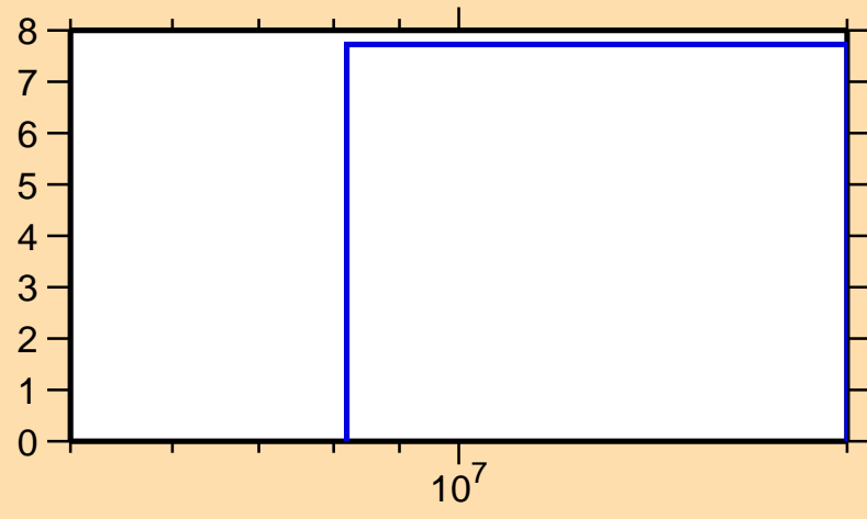
\Delta\sigma/\sigma vs. E for ^{84}\text{Rb}(n,2n)
