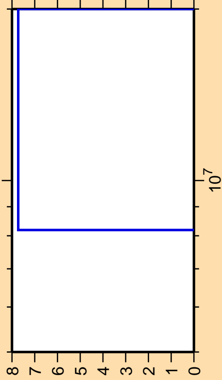
\Delta\sigma/\sigma vs. E for ^{84}\text{Rb}(n,2n)
