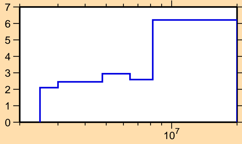
\Delta\sigma/\sigma vs. E for ^{85}\text{Rb}(n,\text{inel.})
