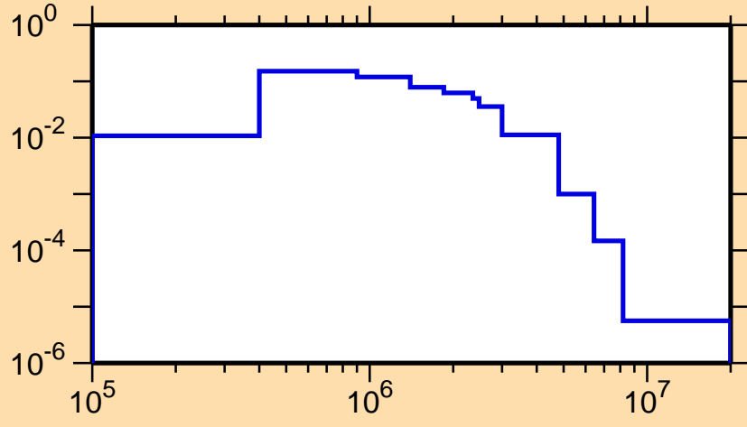
\sigma vs. E for ^{85}\text{Rb}(n,n_2)
