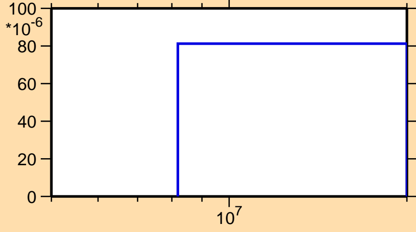
\sigma vs. E for ^{85}\text{Rb}(n,n\alpha)
