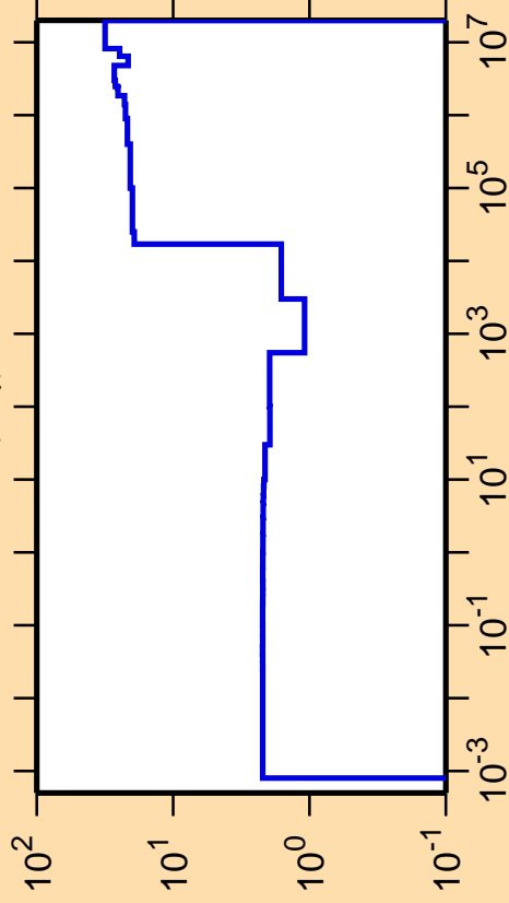
\Delta\sigma/\sigma vs. E for ^{85}\text{Rb}(n,\gamma)
