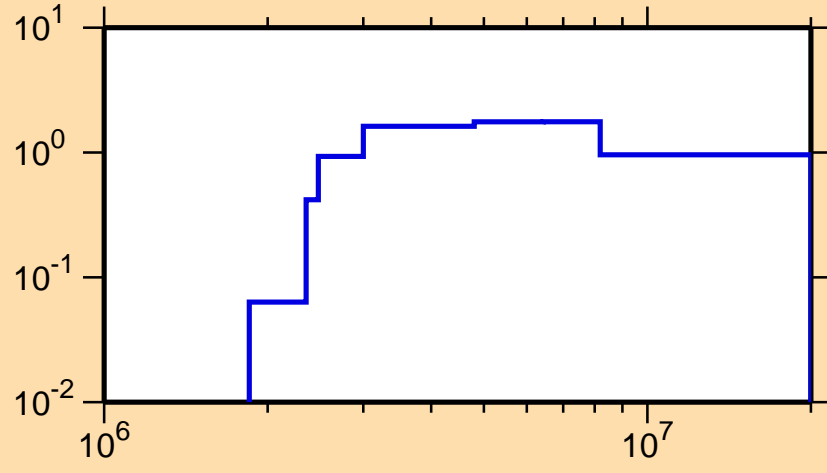
\sigma vs. E for ^{85}\text{Rb}(n,n\text{cont.})
