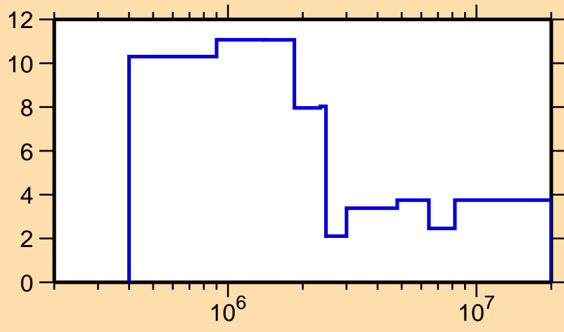
\Delta\sigma/\sigma vs. E for ^{85}\text{Rb}(n,el.)
