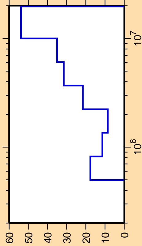
\Delta\sigma/\sigma vs. E for ^{86}\text{Rb}(n,n_2)
