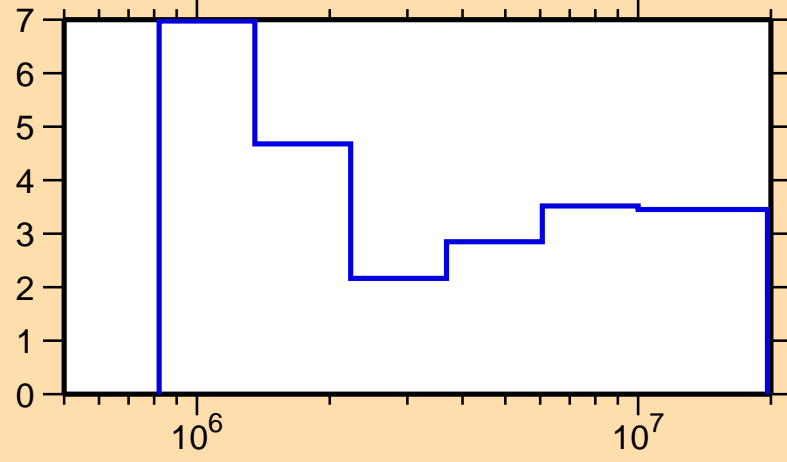
\Delta\sigma/\sigma vs. E for ^{86}\text{Rb}(n,n\text{nonel.})
