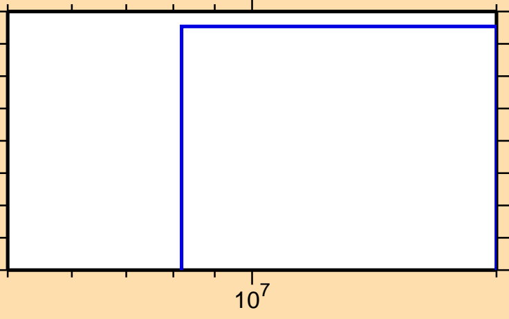
\sigma vs. E for ^{86}\text{Rb}(n,t)
