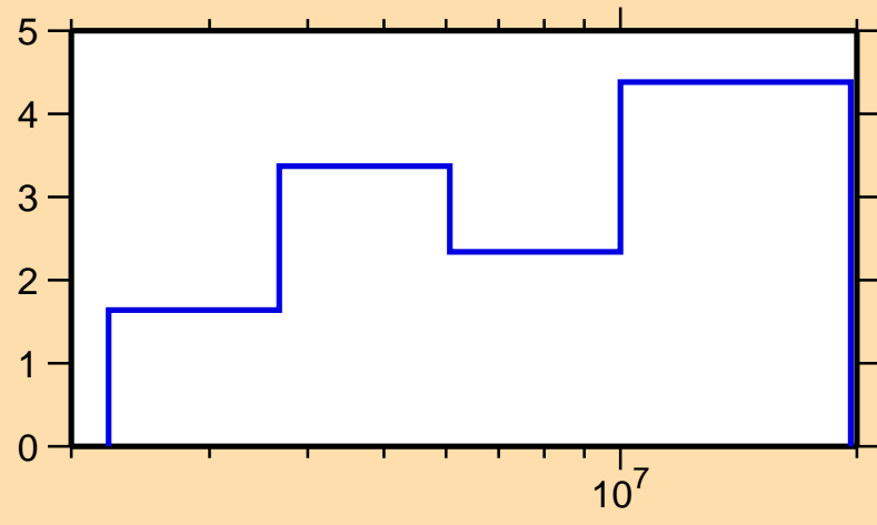
\Delta\sigma/\sigma vs. E for ^{87}\text{Rb}(n,\text{el.})
