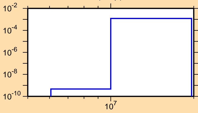
\sigma vs. E for ^{87}\text{Rb}(n,np)
