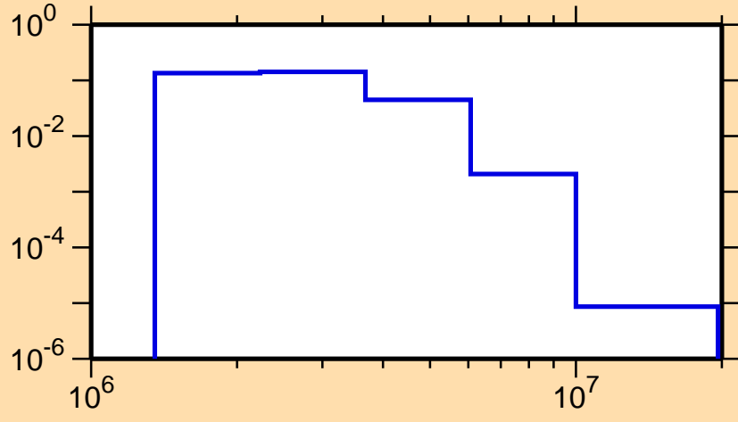
\sigma vs. E for ^{87}\text{Rb}(n,n_3)
