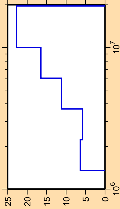
\Delta\sigma/\sigma vs. E for ^{87}\text{Rb}(n,n_3)
