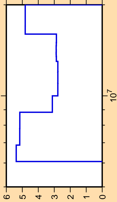
\Delta\sigma/\sigma vs. E for ^{88}\text{Rb}(n,2n)
