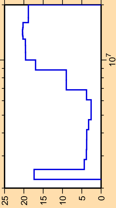
\Delta\sigma/\sigma vs. E for ^{88}\text{Rb}(n,n\text{cont.})
