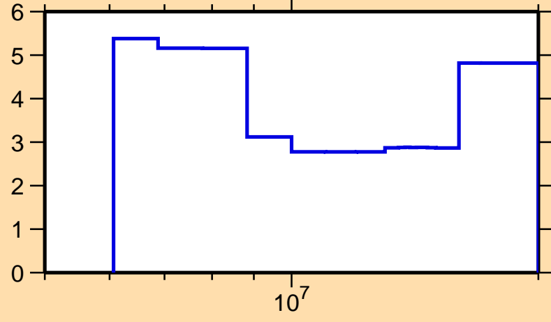
\Delta\sigma/\sigma vs. E for ^{88}\text{Rb}(n,2n)
