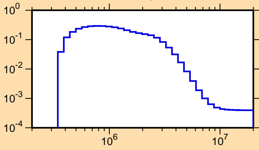
\sigma vs. E for ^{88}\text{Rb}(n,n_4)
