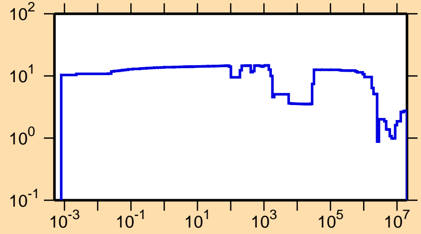
\Delta\sigma/\sigma vs. E for ^{88}\text{Rb}(n,\text{tot.})
