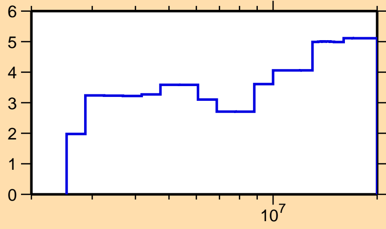
\Delta\sigma/\sigma vs. E for ^{88}\text{Rb}(n,\text{el.})
