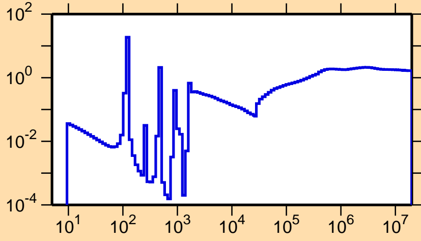
\sigma vs. E for ^{88}\text{Rb}(n,\text{nonel.})
