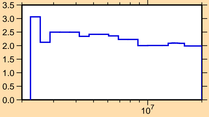
\Delta\sigma/\sigma vs. E for ^{88}\text{Rb}(n,n\text{nonel.})
