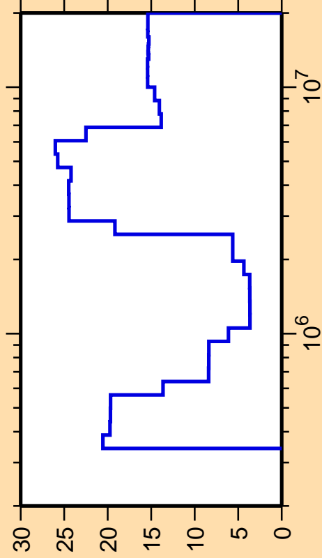
\Delta\sigma/\sigma vs. E for ^{88}\text{Rb}(n,n_4)
