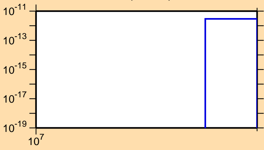
\sigma vs. E for ^{88}\text{Rb}(n,\text{He}3)
