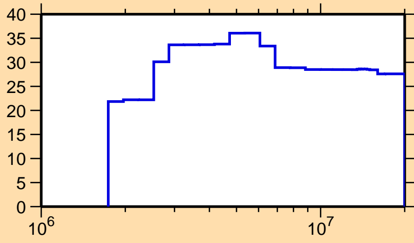
\Delta\sigma/\sigma vs. E for ^{88}\text{Rb}(n,\gamma)
