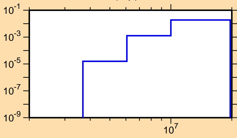
\sigma vs. E for ^{88}\text{Rb}(n,p)
