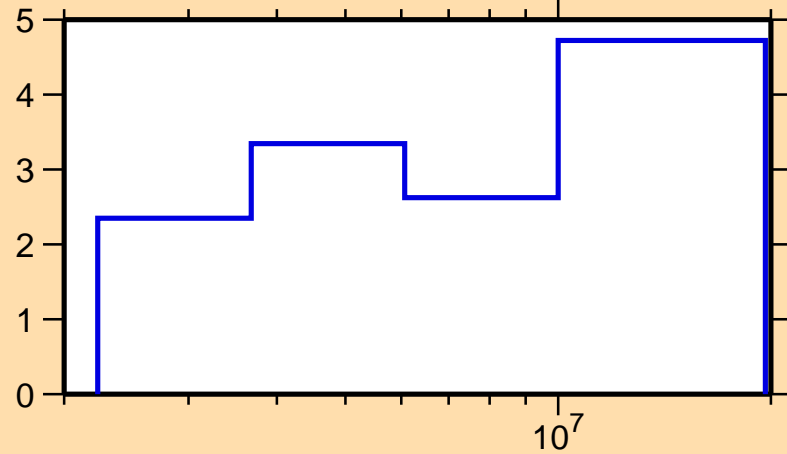
\Delta\sigma/\sigma vs. E for ^{88}\text{Rb}(n,\text{el.})
