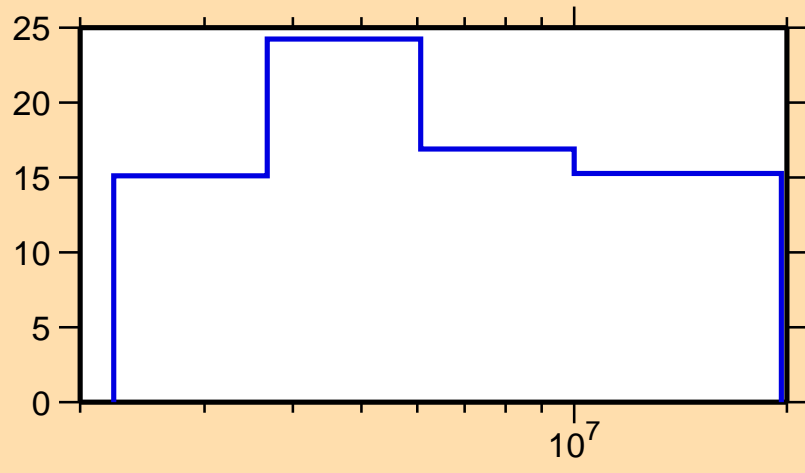
\Delta\sigma/\sigma vs. E for ^{88}\text{Rb}(n,n_1)
