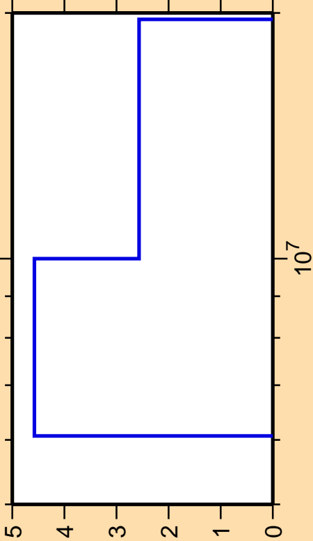
\Delta\sigma/\sigma vs. E for ^{88}\text{Rb}(n,2n)
