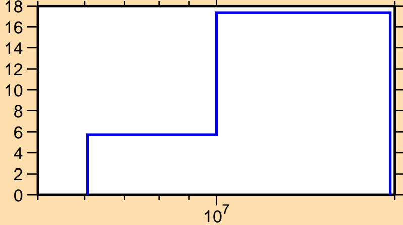
\Delta\sigma/\sigma vs. E for ^{88}\text{Rb}(n,\text{inel.})
