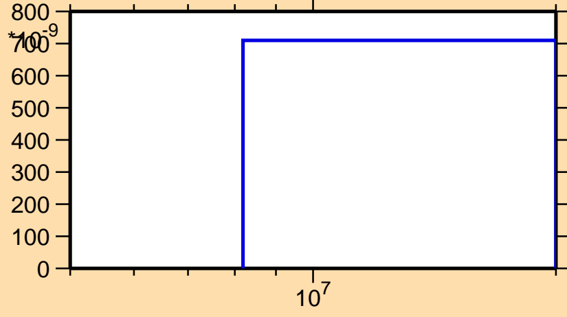
\sigma vs. E for ^{88}\text{Rb}(n,\text{nd})
