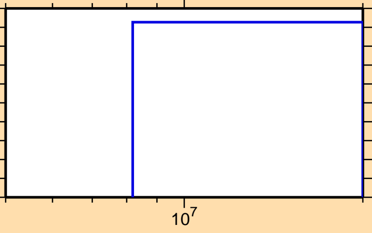
\sigma vs. E for ^{88}\text{Rb}(n,n\alpha)
