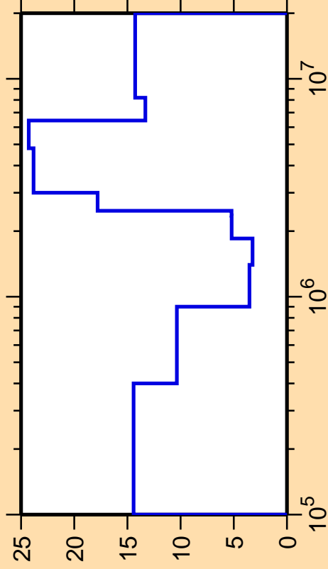
\Delta\sigma/\sigma vs. E for ^{88}\text{Rb}(n,n_2)
