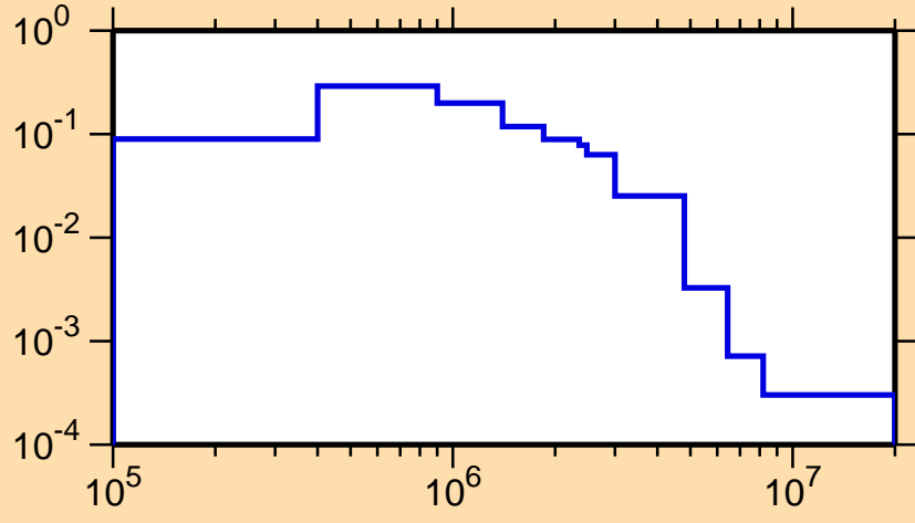
\sigma vs. E for ^{88}\text{Rb}(n,n_2)
