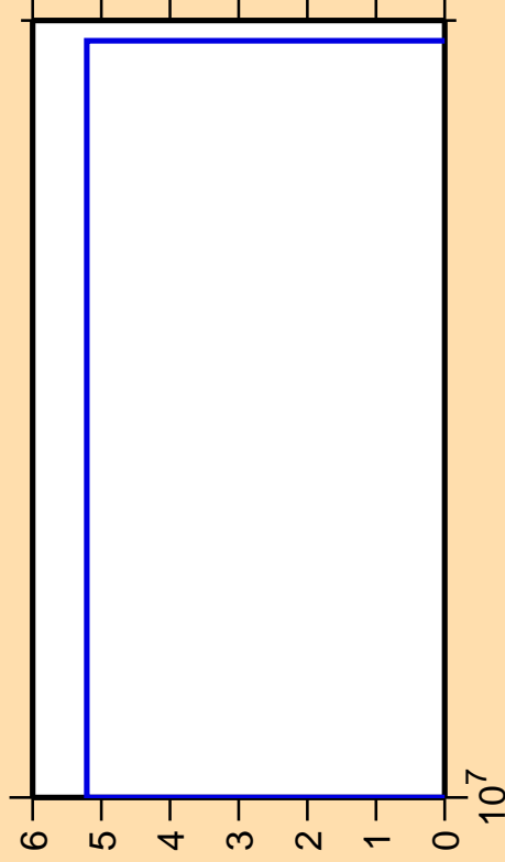
\Delta\sigma/\sigma vs. E for ^{89}\text{Rb}(n,3n)
