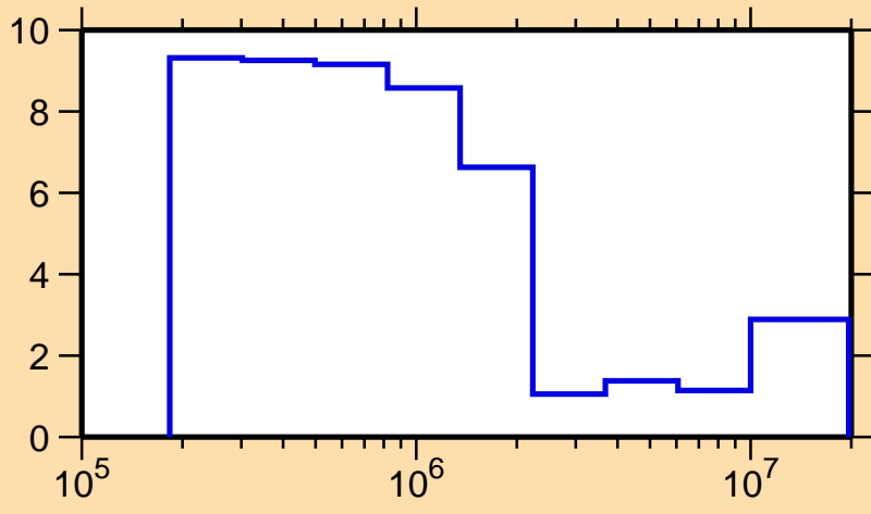
\Delta\sigma/\sigma vs. E for ^{89}\text{Rb}(n,\text{tot.})
