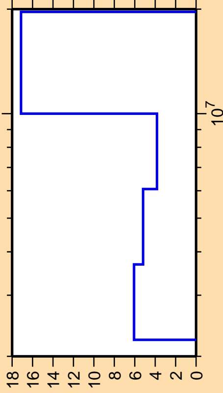
\Delta\sigma/\sigma vs. E for ^{89}\text{Rb}(n,n\text{cont.})
