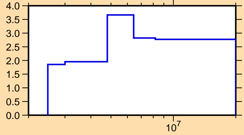
\Delta\sigma/\sigma vs. E for ^{89}\text{Rb}(n,n\text{nonel.})
