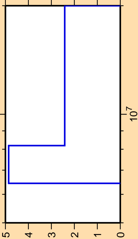
\Delta\sigma/\sigma vs. E for ^{89}\text{Rb}(n,2n)
