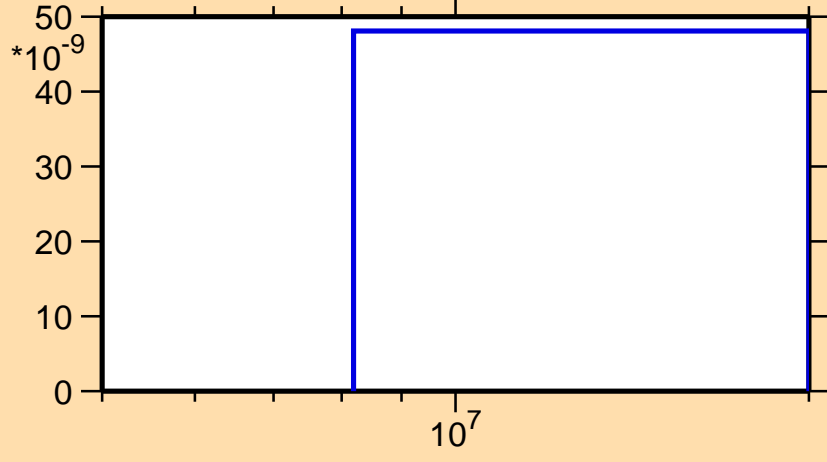
\sigma vs. E for ^{89}\text{Rb}(n,nt)
