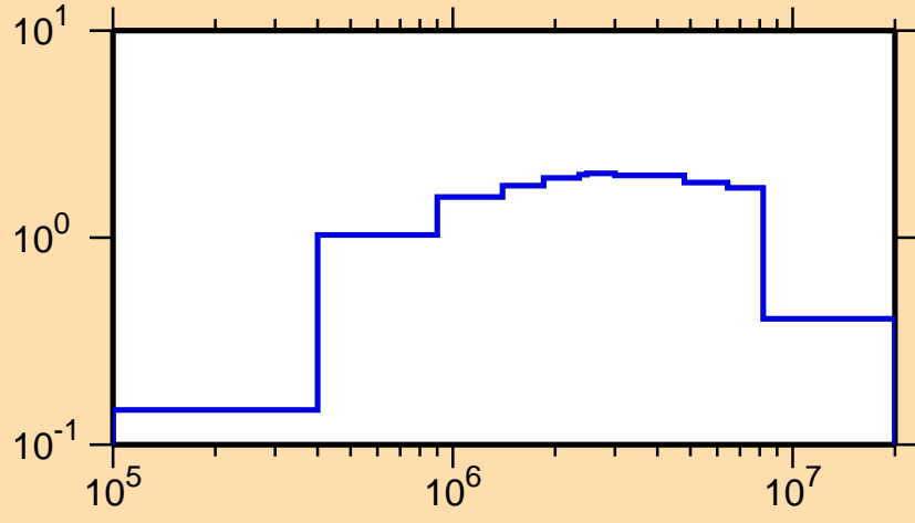
\sigma vs. E for ^{89}\text{Rb}(n,\text{inel.})
