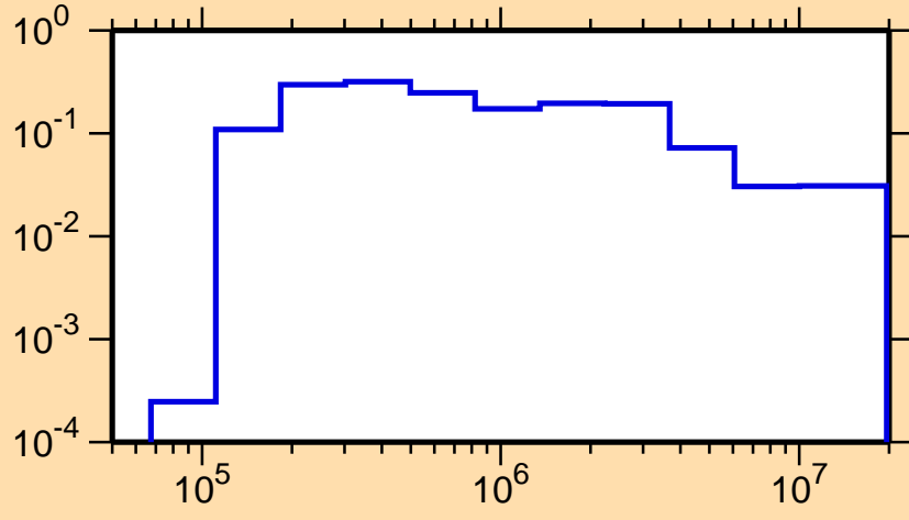
\sigma vs. E for ^{90}\text{Rb}(n,n_1)
