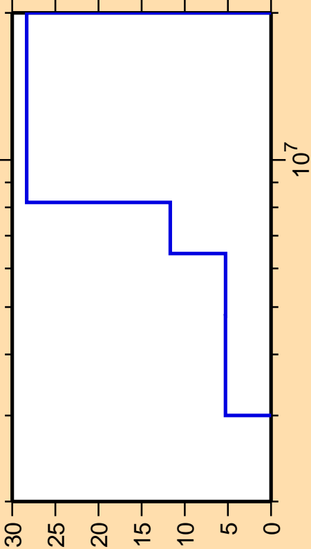
\Delta\sigma/\sigma vs. E for ^{90}\text{Rb}(n,n\text{cont.})
