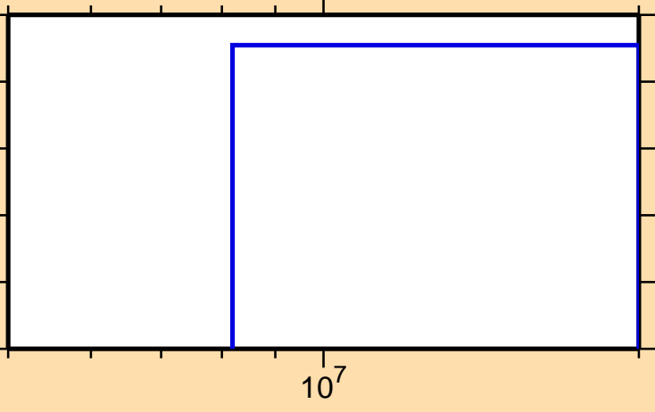
\sigma vs. E for ^{90}\text{Rb}(n,2np)
