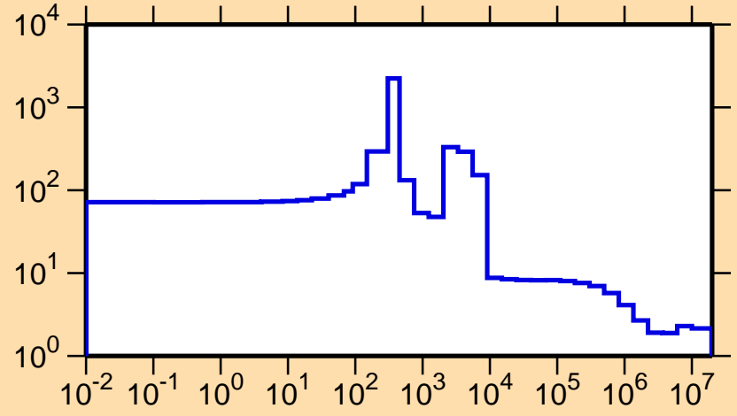
\sigma vs. E for ^{91}\text{Rb}(n,\text{el.})
