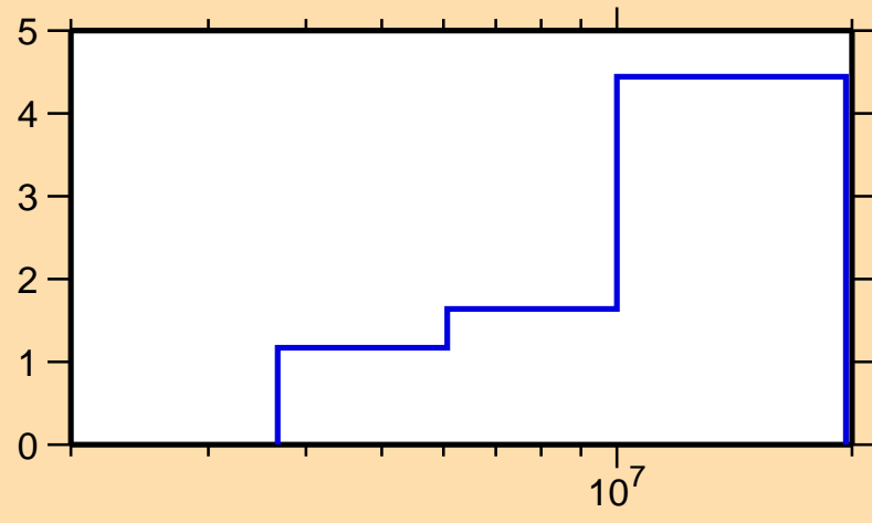
\Delta\sigma/\sigma vs. E for ^{91}\text{Rb}(n,\text{tot.})
