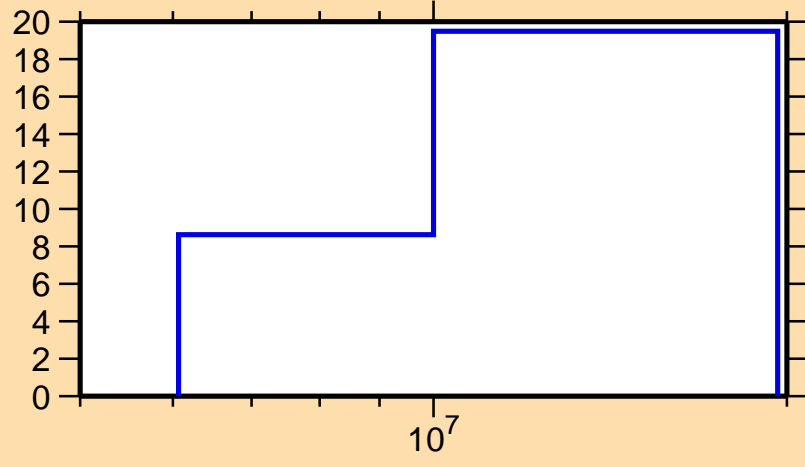
\Delta\sigma/\sigma vs. E for ^{91}\text{Rb}(n,ncont.)
