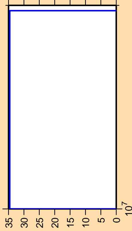
\Delta\sigma/\sigma vs. E for ^{91}\text{Rb}(n,2n\alpha)
