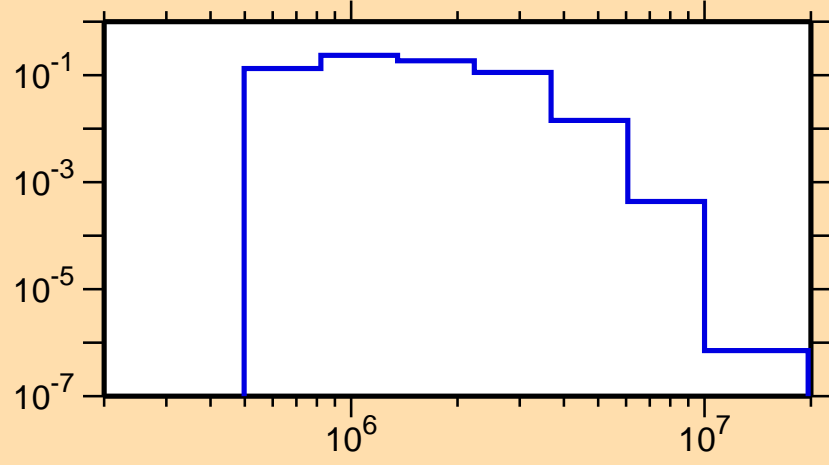
\sigma vs. E for ^{91}\text{Rb}(n,n_3)
