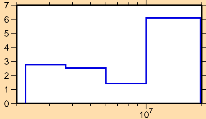
\Delta\sigma/\sigma vs. E for ^{91}\text{Rb}(n,\text{el.})
