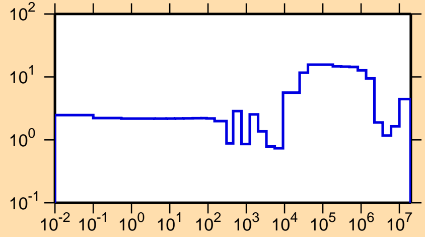
\Delta\sigma/\sigma vs. E for ^{91}\text{Rb}(n,\text{tot.})
