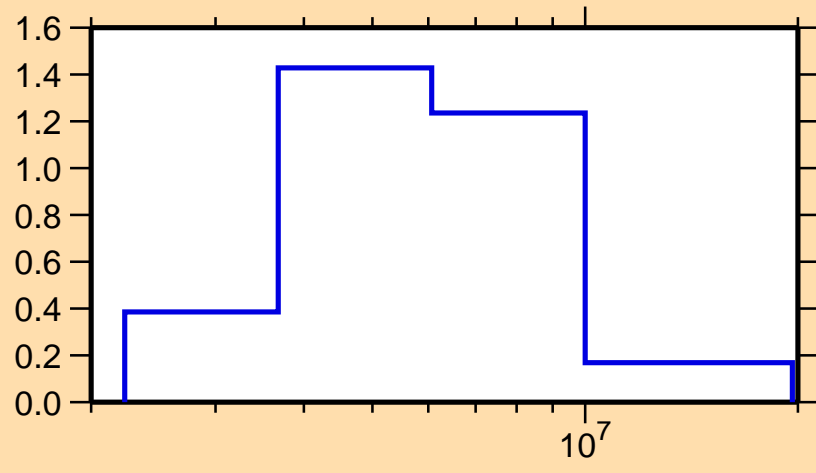
\sigma vs. E for ^{91}\text{Rb}(n,n\text{cont.})
