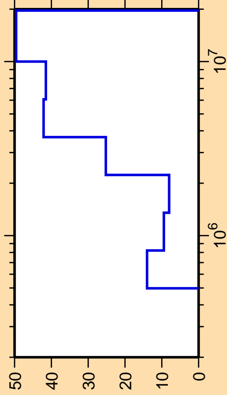
\Delta\sigma/\sigma vs. E for ^{91}\text{Rb}(n,n_2)
