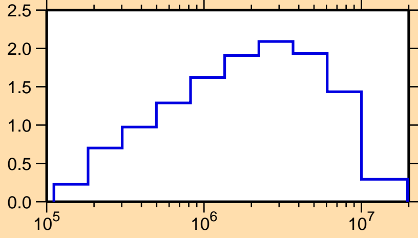
\sigma vs. E for ^{91}\text{Rb}(n,\text{inel.})
