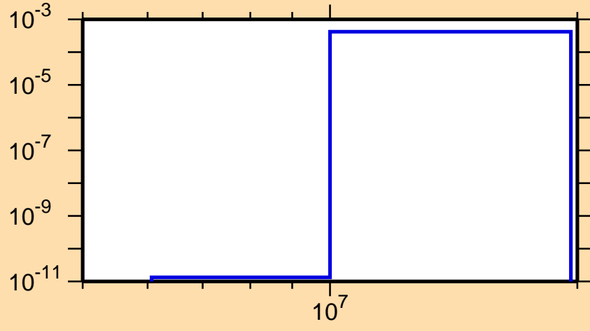
\sigma vs. E for ^{91}\text{Rb}(n,d)
