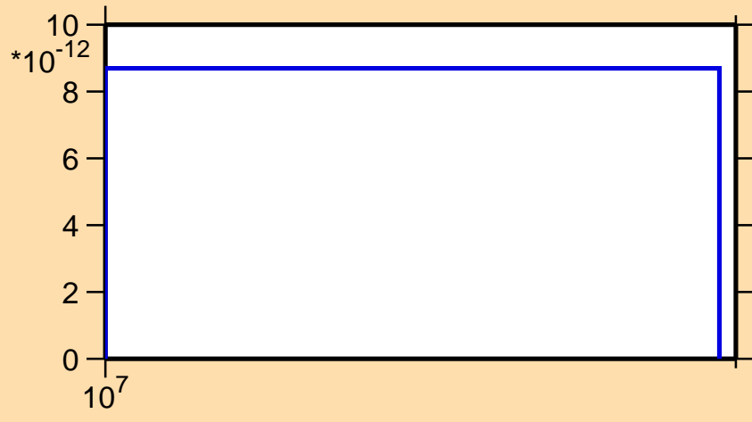
\sigma vs. E for ^{91}\text{Rb}(n,2n\alpha)
