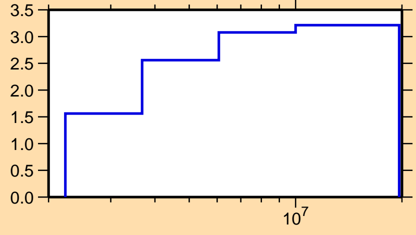
\Delta\sigma/\sigma vs. E for ^{91}\text{Rb}(n,n\text{nonel.})
