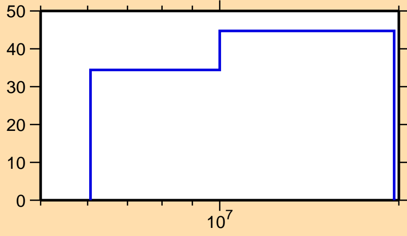
\Delta\sigma/\sigma vs. E for ^{91}\text{Rb}(n,\gamma)
