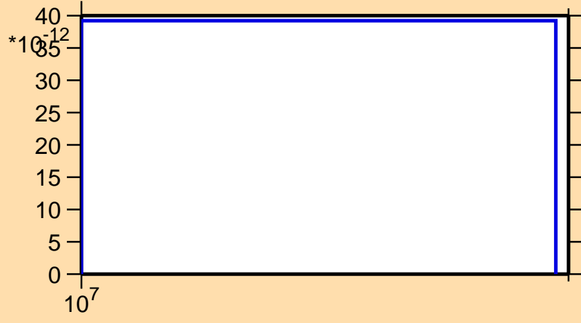
\sigma vs. E for ^{91}\text{Rb}(n,2np)
