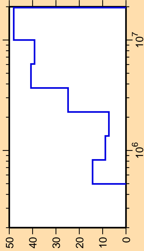
\Delta\sigma/\sigma vs. E for ^{91}\text{Rb}(n,n_3)
