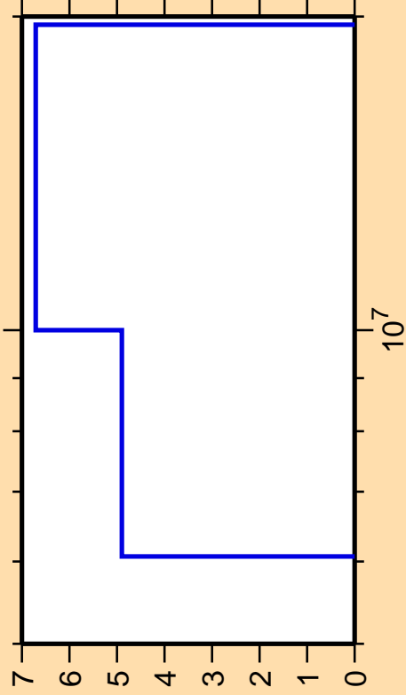
\Delta\sigma/\sigma vs. E for ^{91}\text{Rb}(n,2n)
