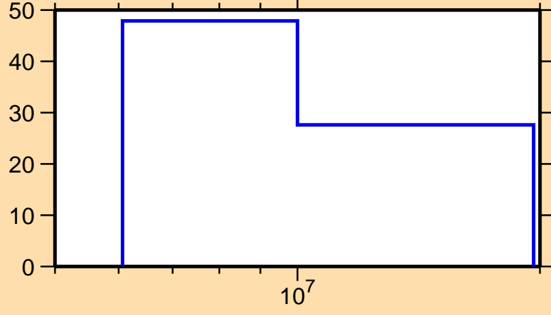
\Delta\sigma/\sigma vs. E for ^{91}\text{Rb}(n,p)
