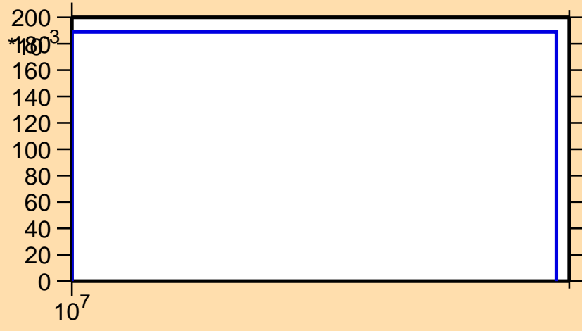
\sigma vs. E for ^{91}\text{Rb}(n,3n)
