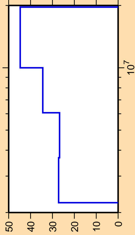
\Delta\sigma/\sigma vs. E for ^{91}\text{Rb}(n,\gamma)
