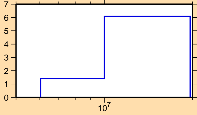
\Delta\sigma/\sigma vs. E for ^{91}\text{Rb}(n,\text{el.})
