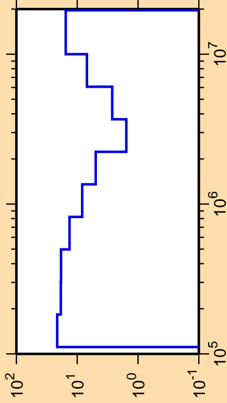
\Delta\sigma/\sigma vs. E for ^{91}\text{Rb}(n,\text{inel.})
