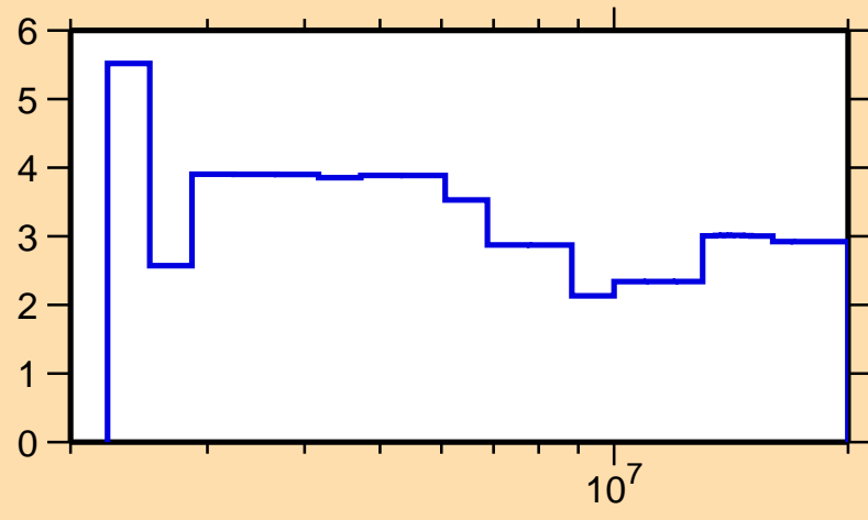
\Delta\sigma/\sigma vs. E for ^{92}\text{Rb}(n,\text{tot.})
