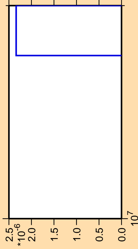
\Delta\sigma/\sigma vs. E for ^{92}\text{Rb} (mt 11)
