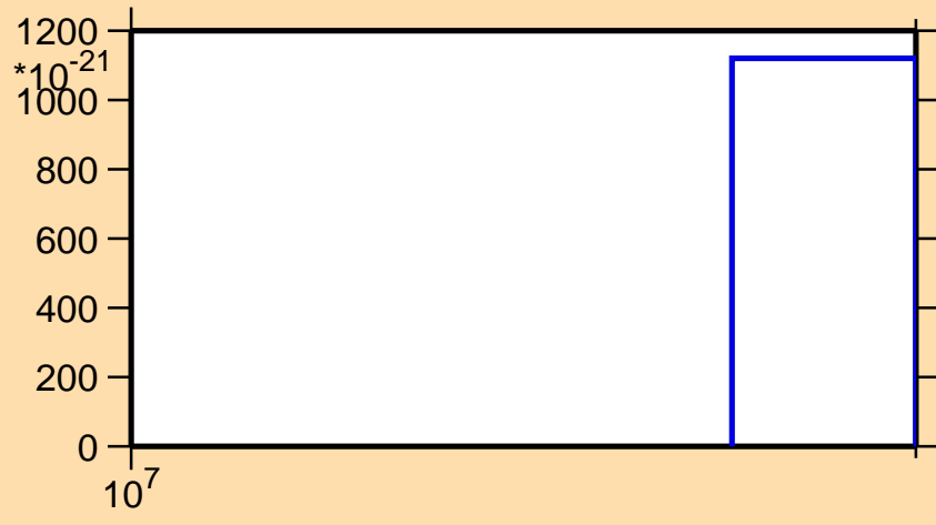
\sigma vs. E for ^{92}\text{Rb} (mt 11)
