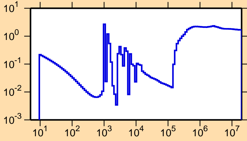
\sigma vs. E for ^{92}\text{Rb}(n,\text{nonel.})
