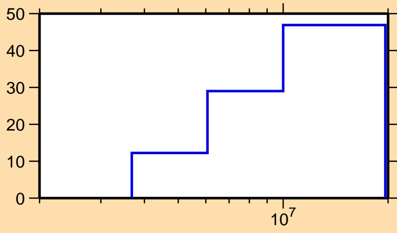
\Delta\sigma/\sigma vs. E for ^{92}\text{Rb}(n,ncont.)
