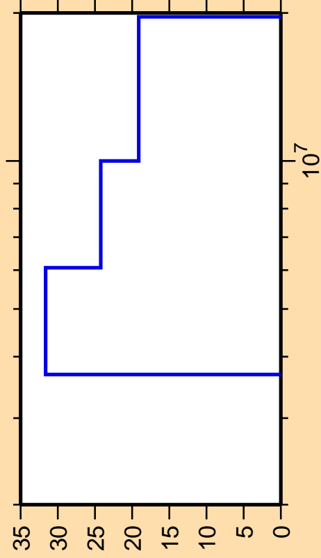
\Delta\sigma/\sigma vs. E for ^{92}\text{Rb}(n,n_1)
