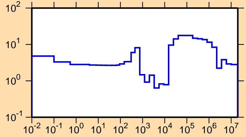
\Delta\sigma/\sigma vs. E for ^{92}\text{Rb}(n,\text{tot.})
