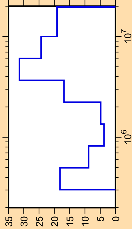
\Delta\sigma/\sigma vs. E for ^{92}\text{Rb}(n,n_4)
