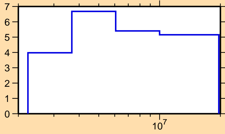
\Delta\sigma/\sigma vs. E for ^{92}\text{Rb}(n,\text{el.})
