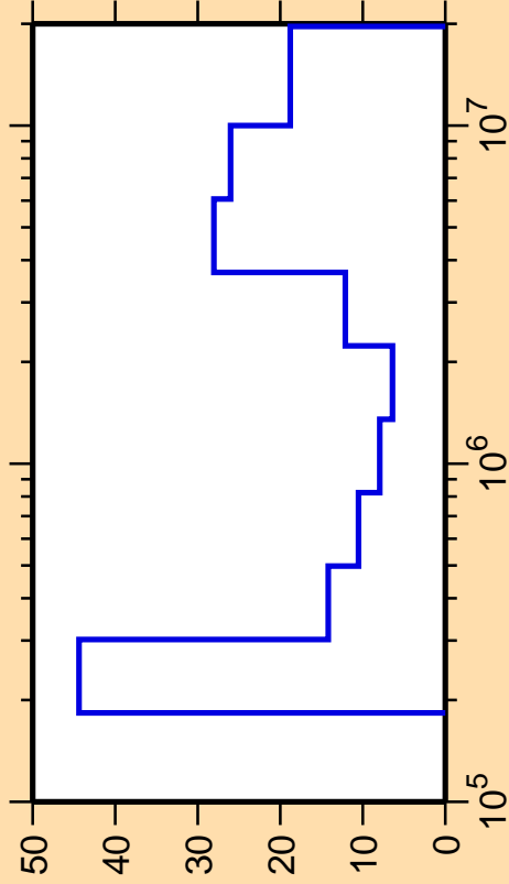
\Delta\sigma/\sigma vs. E for ^{92}\text{Rb}(n,n_2)
