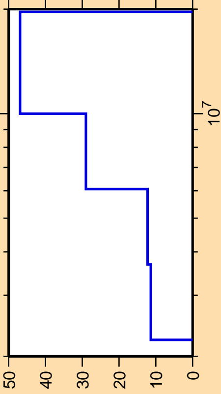
\Delta\sigma/\sigma vs. E for ^{92}\text{Rb}(n,n\text{cont.})
