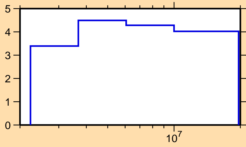
\Delta\sigma/\sigma vs. E for ^{92}\text{Rb}(n,n\text{nonel.})
