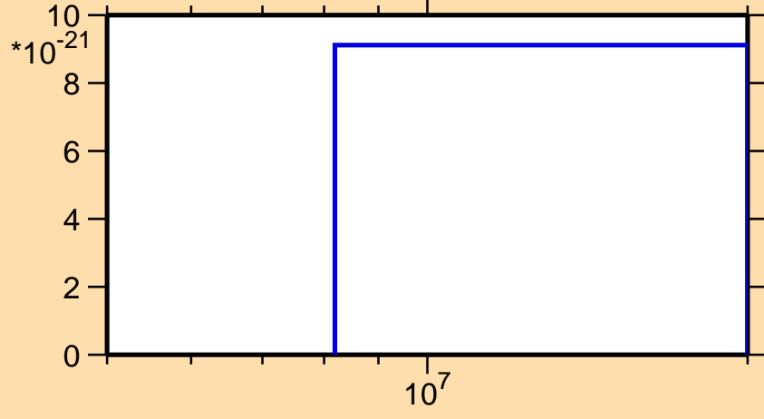
\sigma vs. E for ^{92}\text{Rb} (mt 11)
