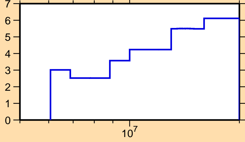
\Delta\sigma/\sigma vs. E for ^{93}\text{Rb}(n,\text{tot.})
