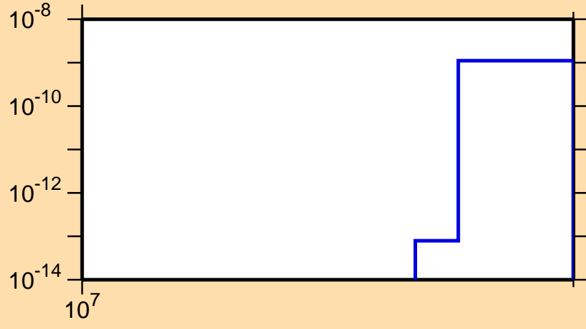
\sigma vs. E for ^{93}\text{Rb}(n,2n\alpha)
