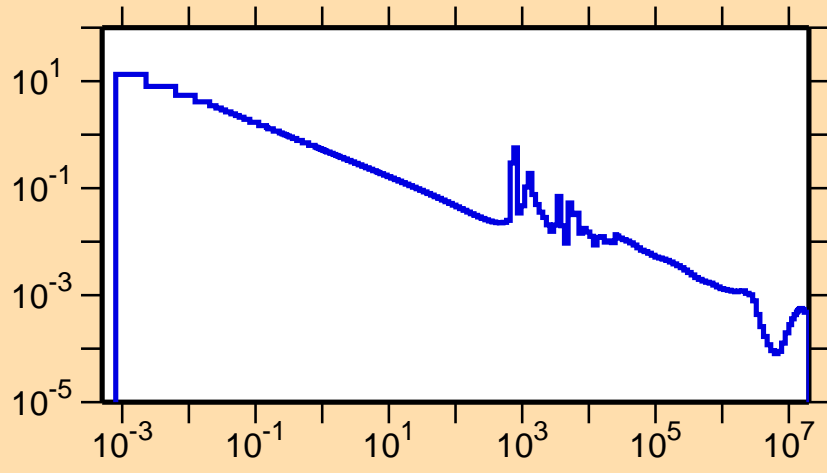
\sigma vs. E for ^{93}\text{Rb}(n,\gamma)
