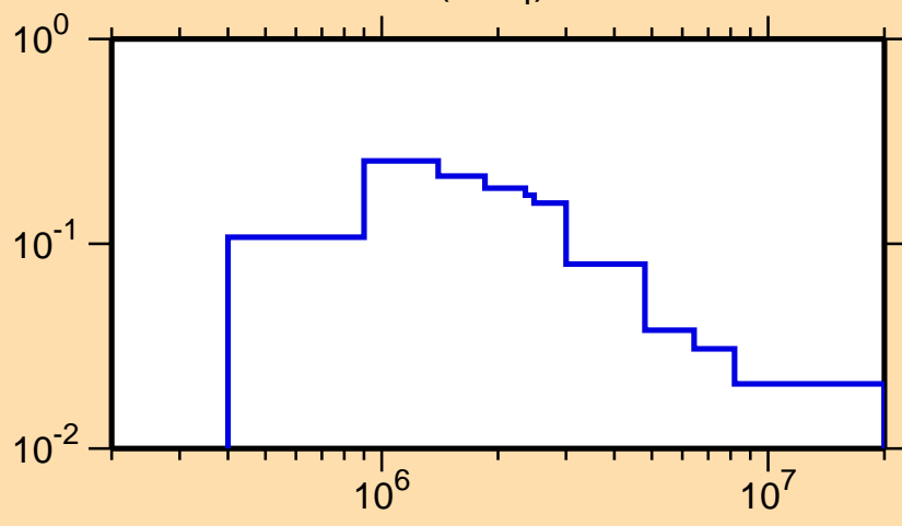
\sigma vs. E for ^{93}\text{Rb}(n,n_4)
