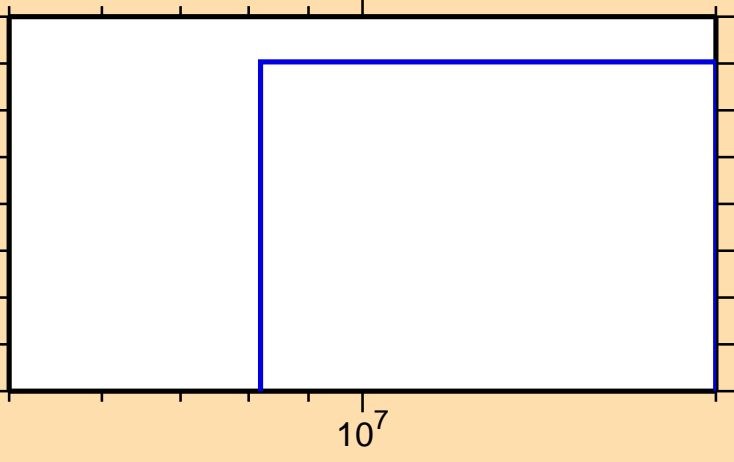
\sigma vs. E for ^{93}\text{Rb}(n,\text{nd})
