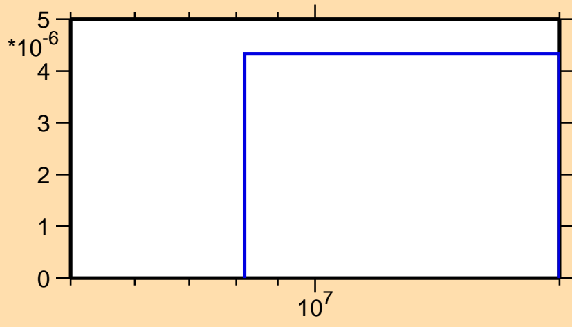
\sigma vs. E for ^{93}\text{Rb}(n,n\alpha)
