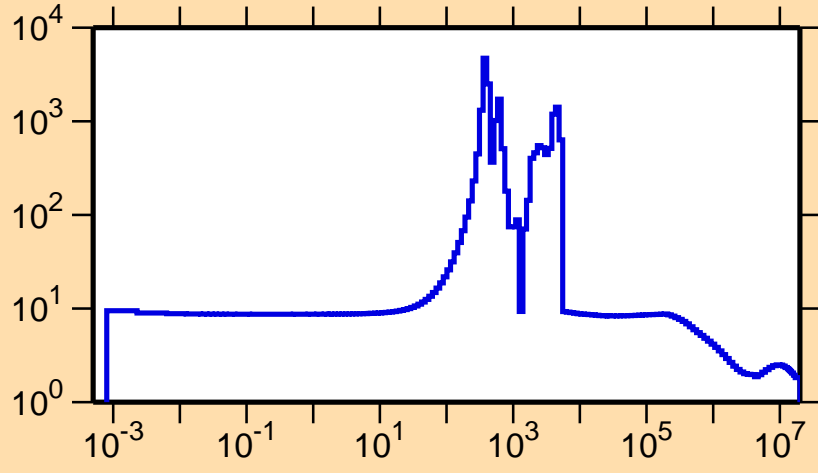
\sigma vs. E for ^{94}\text{Rb}(n,\text{el.})
