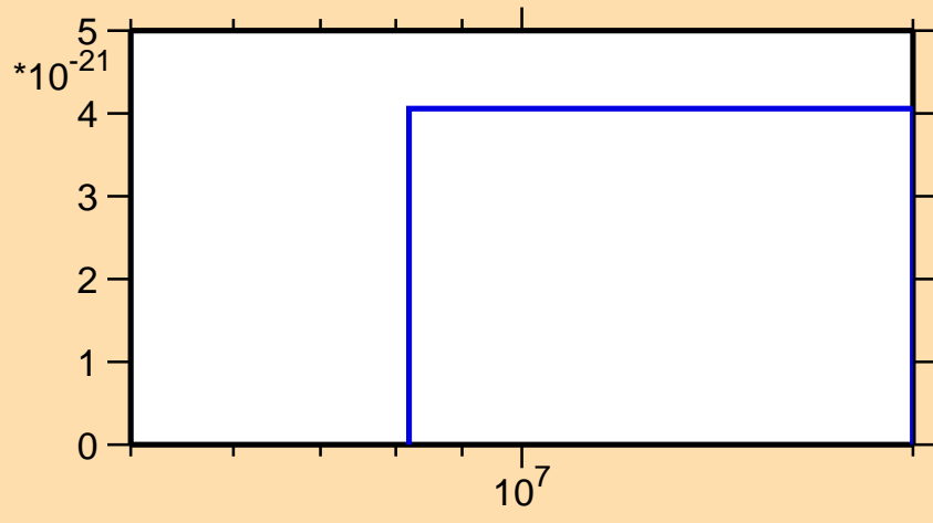
\sigma vs. E for ^{94}\text{Rb} (mt 11)
