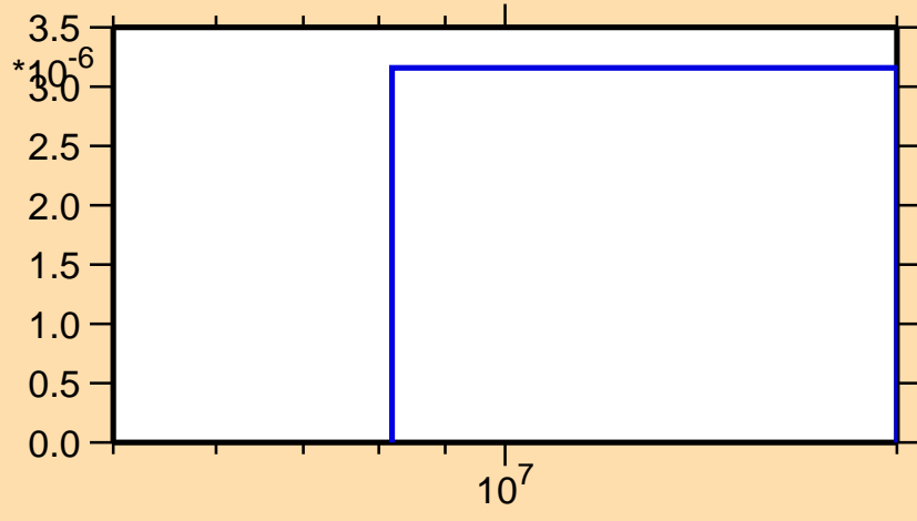
\sigma vs. E for ^{94}\text{Rb}(n,n\alpha)
