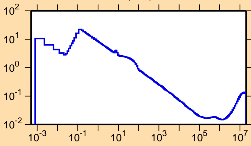
\sigma vs. E for ^{165}\text{Re}(n,\alpha)
