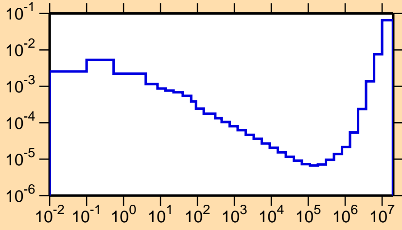
\sigma vs. E for ^{165}\text{Re}(n, p\alpha)
