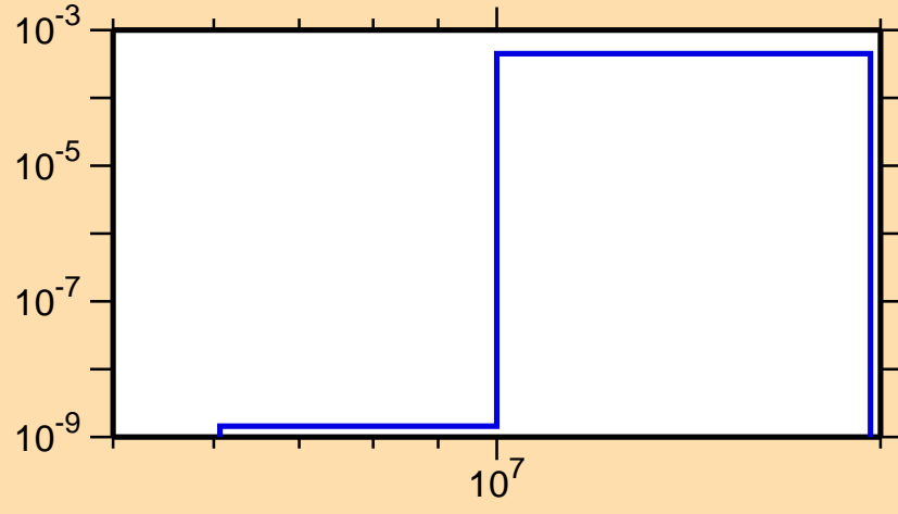
\sigma vs. E for ^{165}\text{Re}(n,t)
