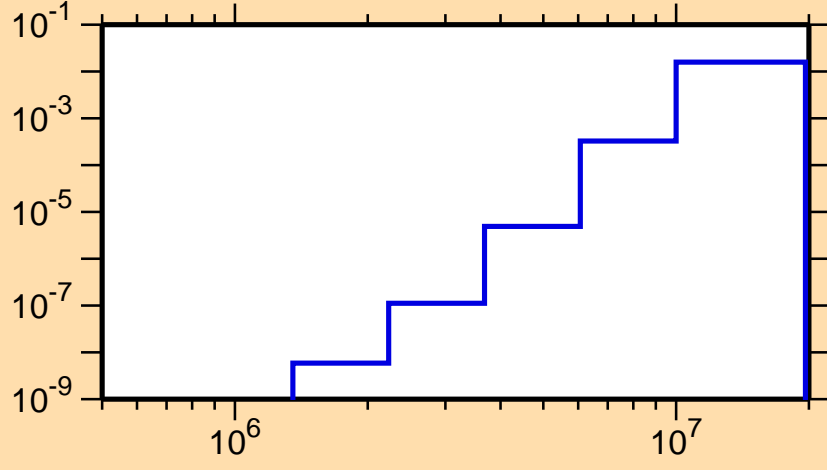
\sigma vs. E for ^{165}\text{Re}(n,d)
