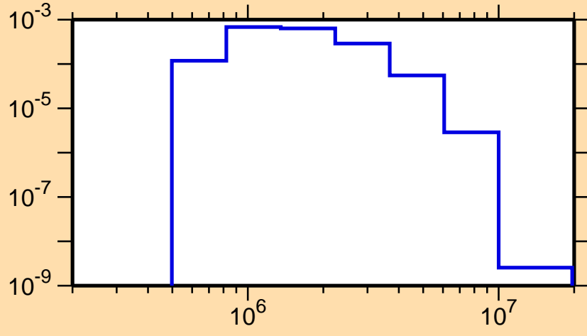
\sigma vs. E for ^{165}\text{Re}(n,n_4)
