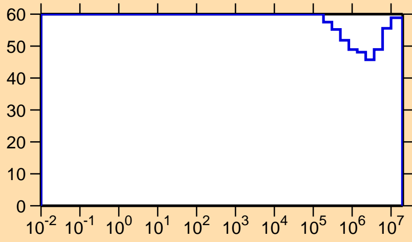
\Delta\sigma/\sigma vs. E for ^{165}\text{Re}(n,p)
