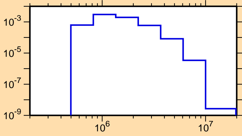
\sigma vs. E for ^{165}\text{Re}(n,n_3)
