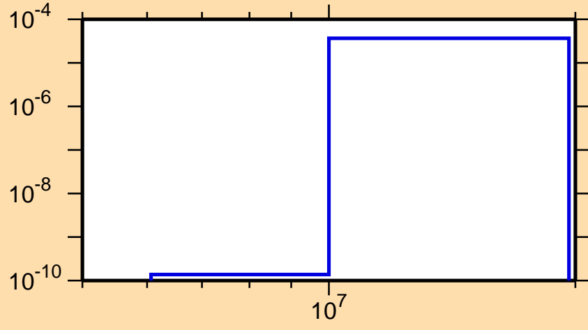
\sigma vs. E for ^{165}\text{Re}(n,\text{pd})
